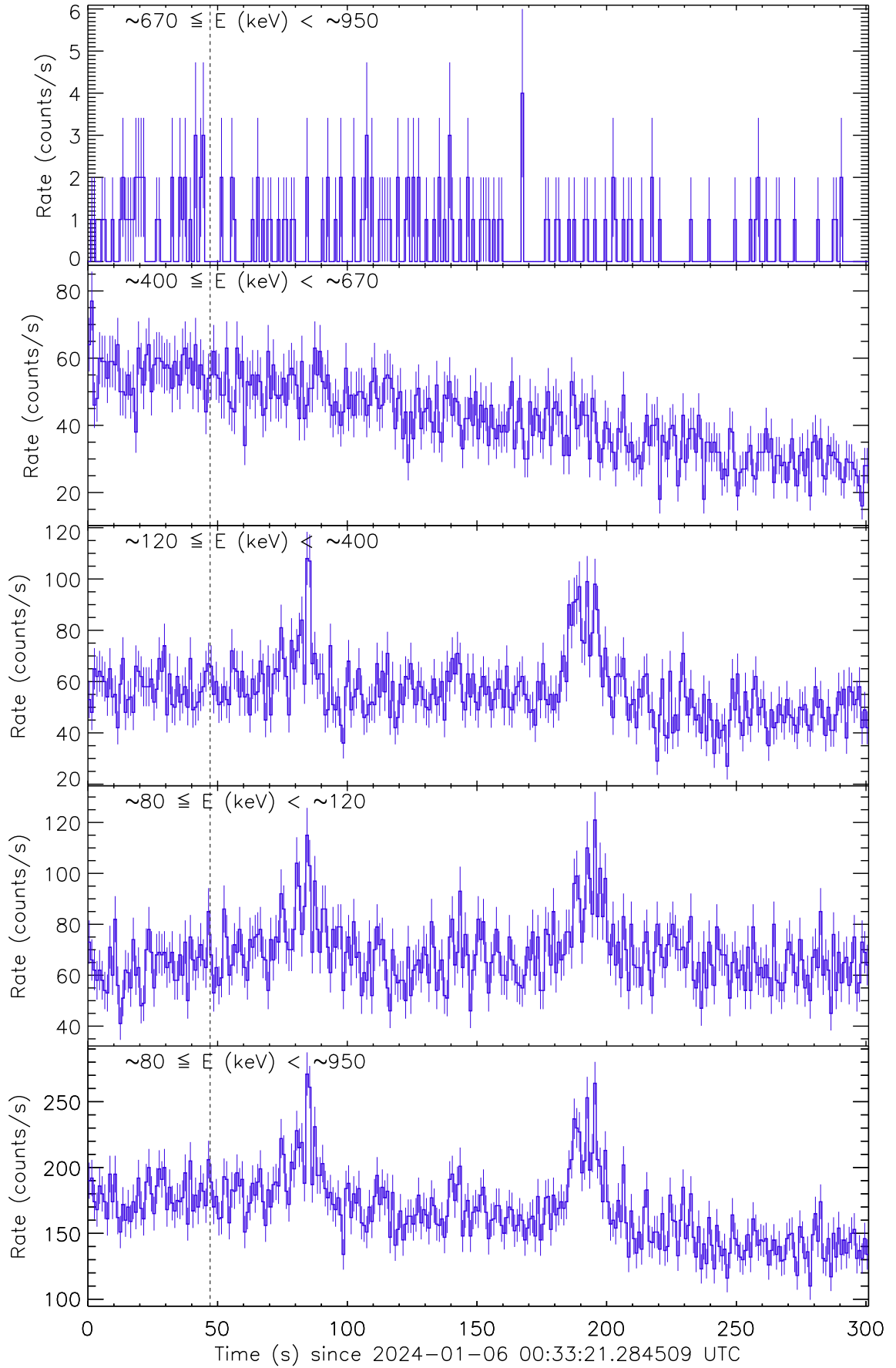
Figure 1: Raw count rate curve of GRB 240106A. The vertical dashed line marks the trigger time by Fermi/GBM.
