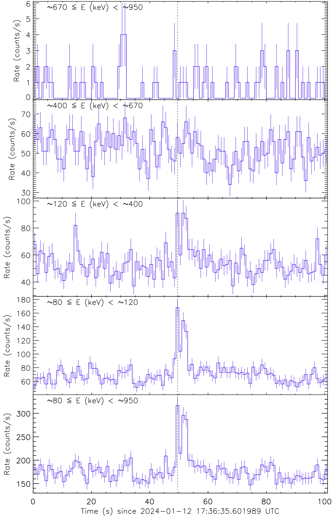
Figure 1: Raw count rate curve of GRB 240112C. The vertical dashed line marks the trigger time by Fermi/GBM.
