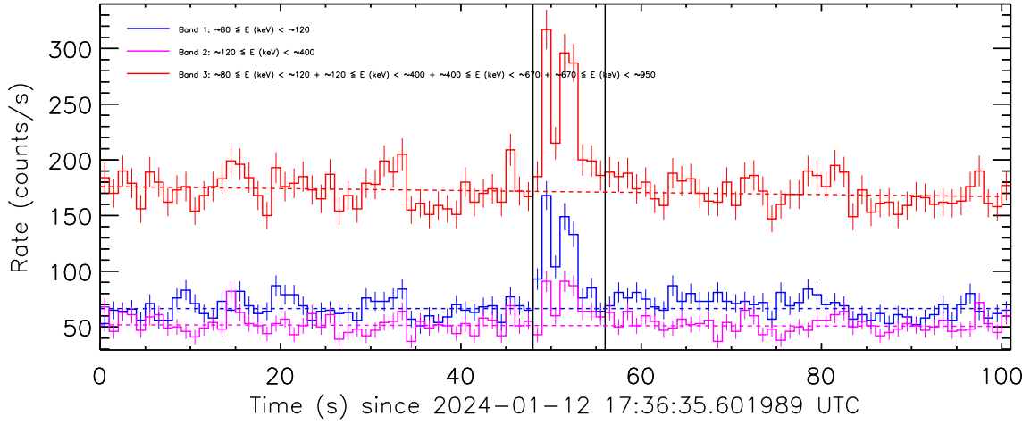
Figure 2: Background fit by a linear function. Pre-burst and post-burst intervals were used for the background fit which are delimited by the vertical solid lines.
