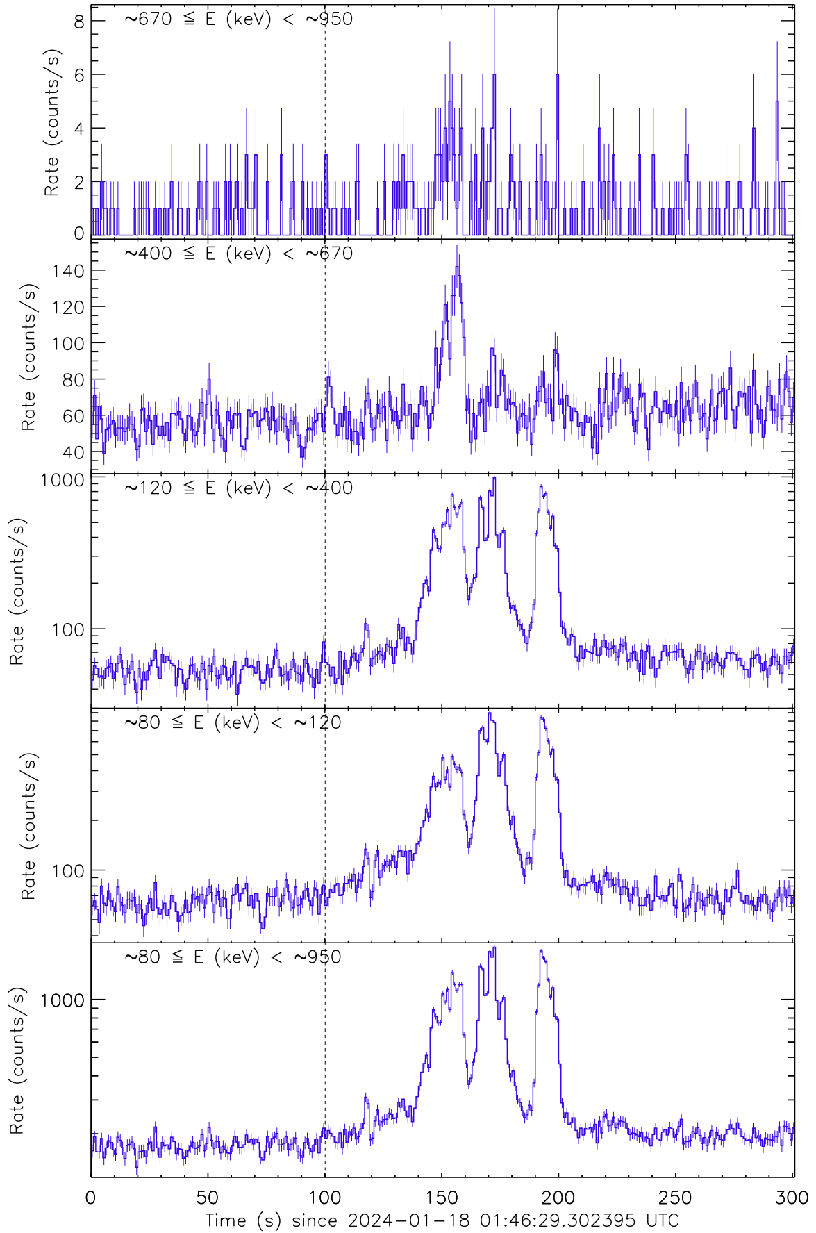
Figure 1: Raw count rate curve of GRB 240118A. The vertical dashed line marks the trigger time by Fermi/GBM.
