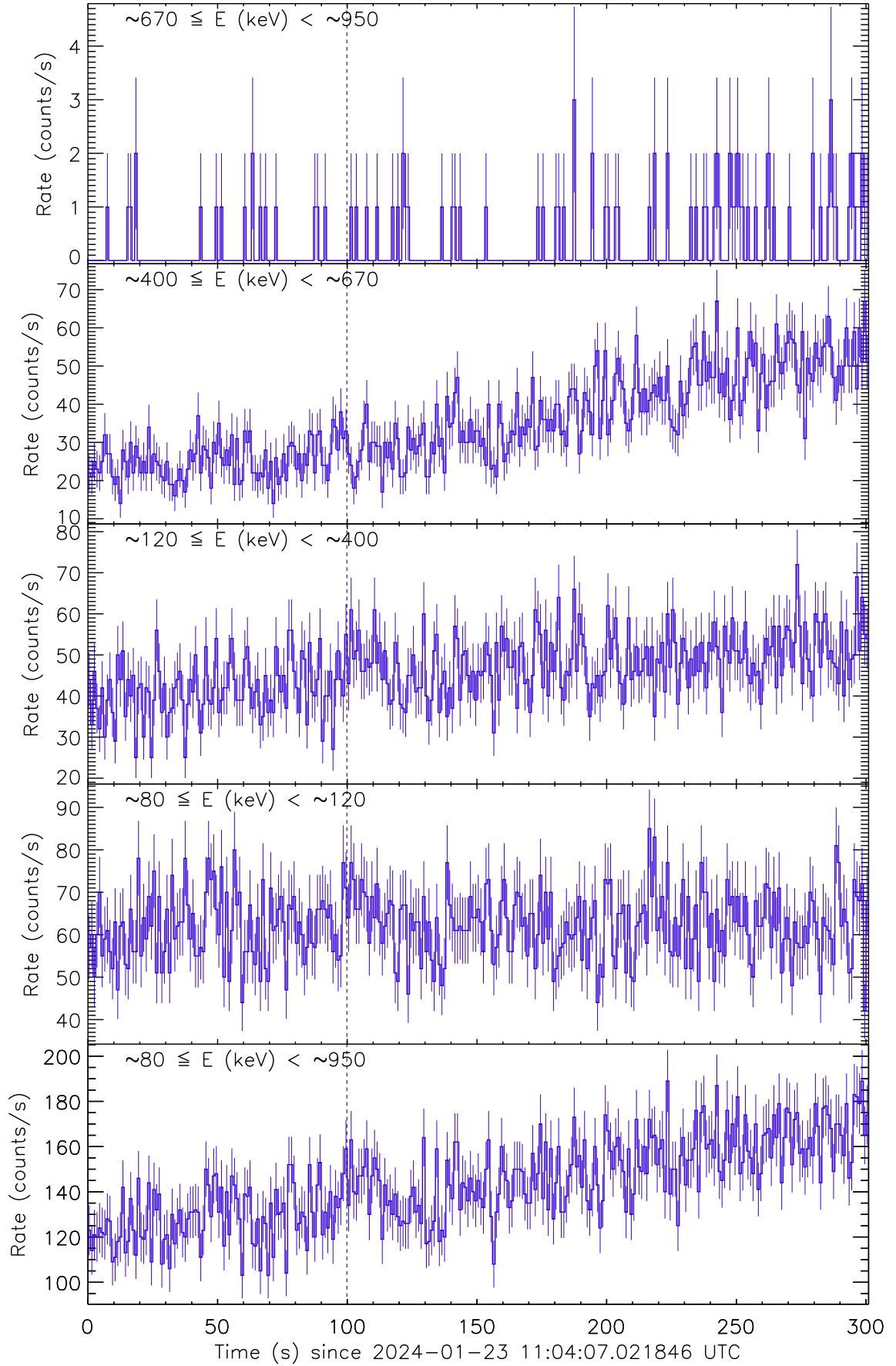
Figure 1: Raw count rate curve of GRB 240123A. The vertical dashed line marks the trigger time by Swift/BAT.
