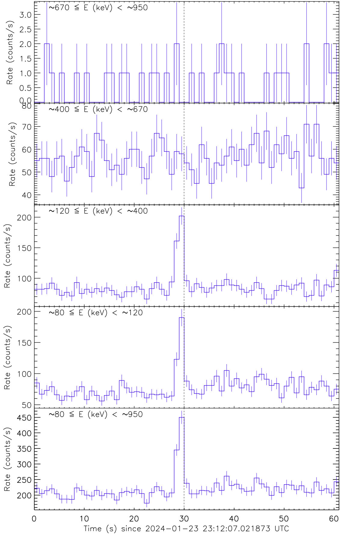
Figure 1: Raw count rate curve of GRB 240123C. The vertical dashed line marks the trigger time by AstroSat.
