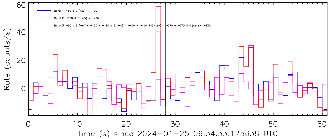
Figure 3: Background-subtracted count rate curve.
