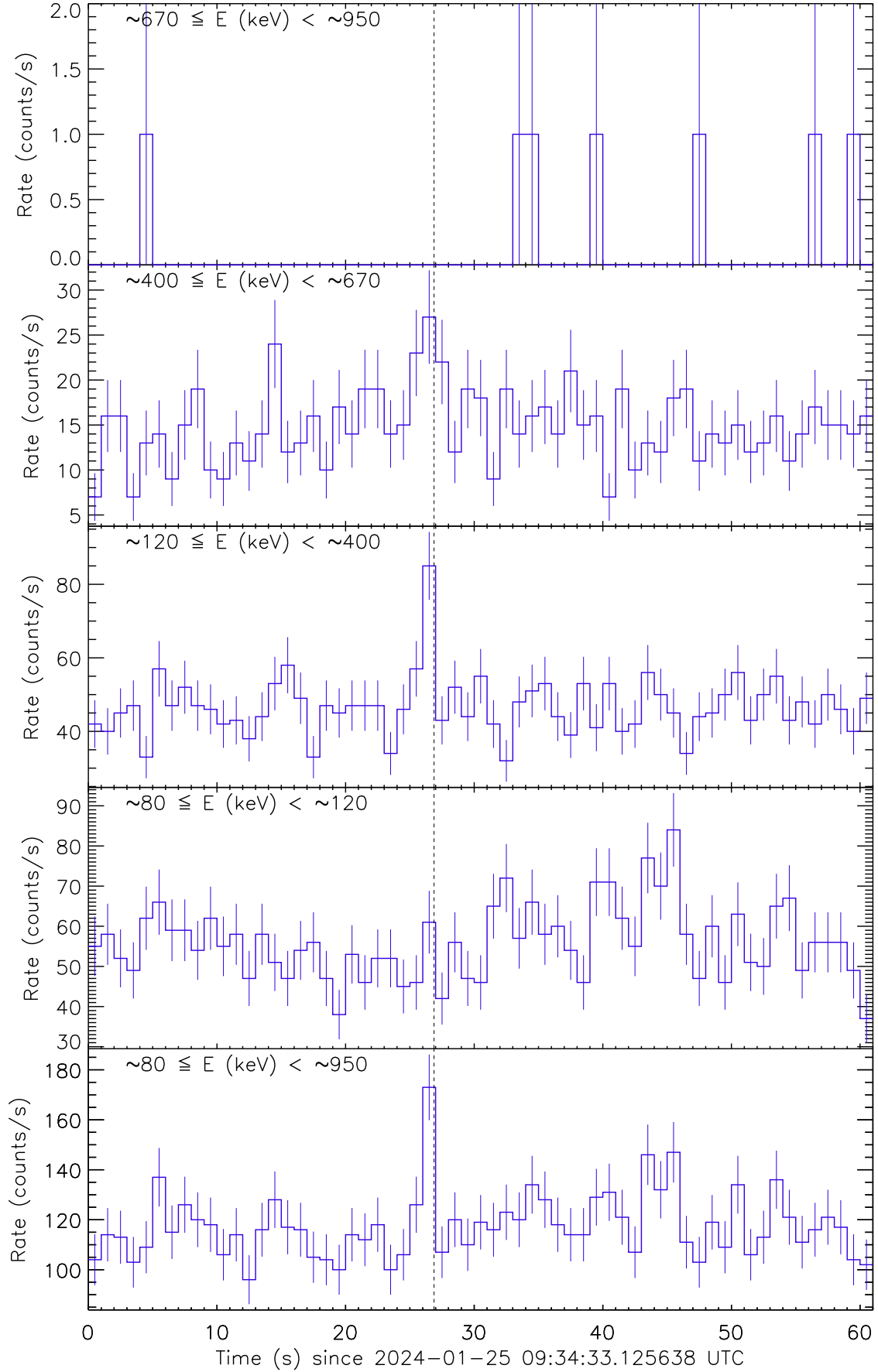
Figure 1: Raw count rate curve of GRB 240125A. The vertical dashed line marks the trigger time by AstroSat.
