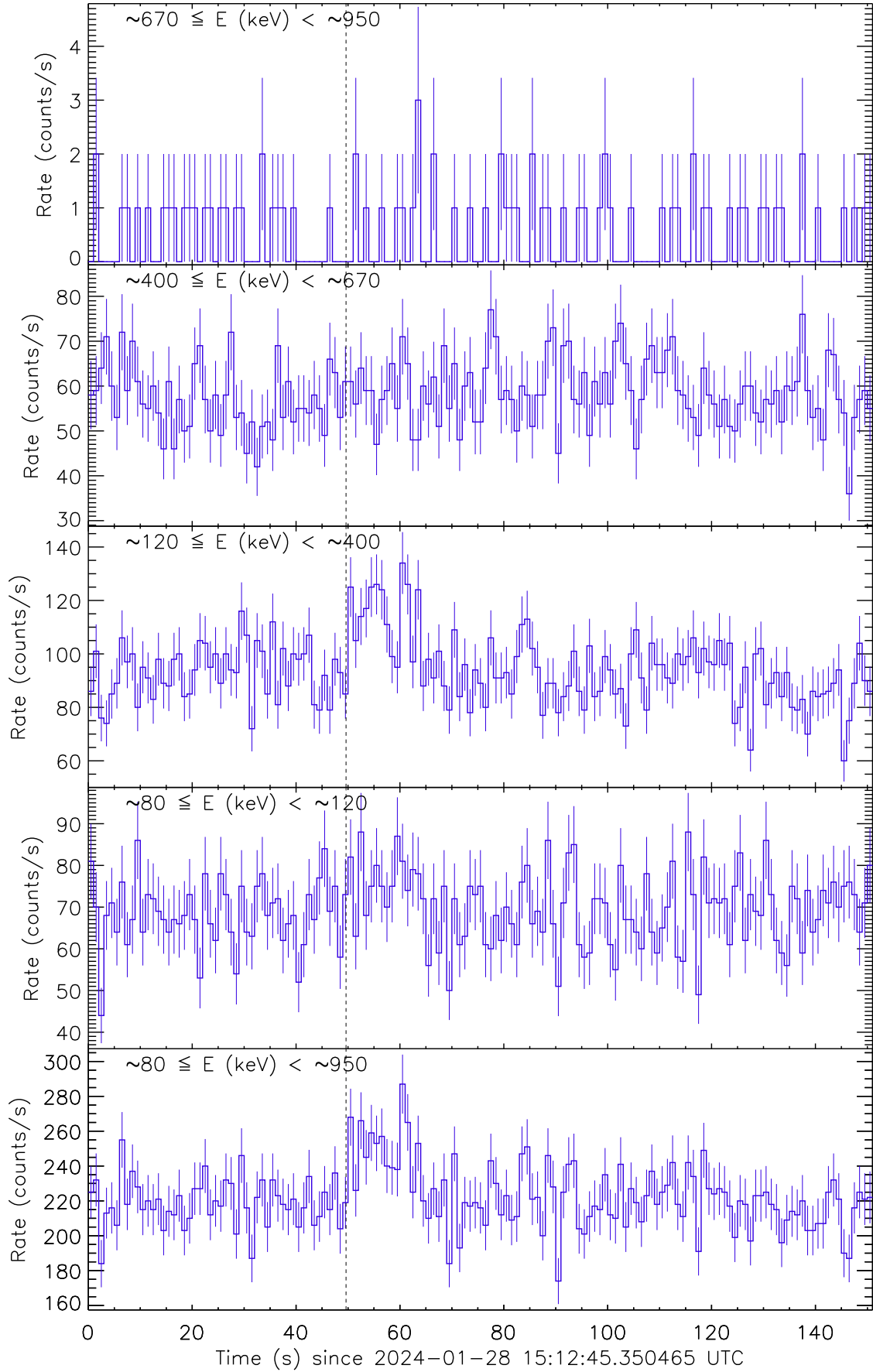
Figure 1: Raw count rate curve of GRB 240128A. The vertical dashed line marks the trigger time by INTEGRAL/SPI-ACS.
