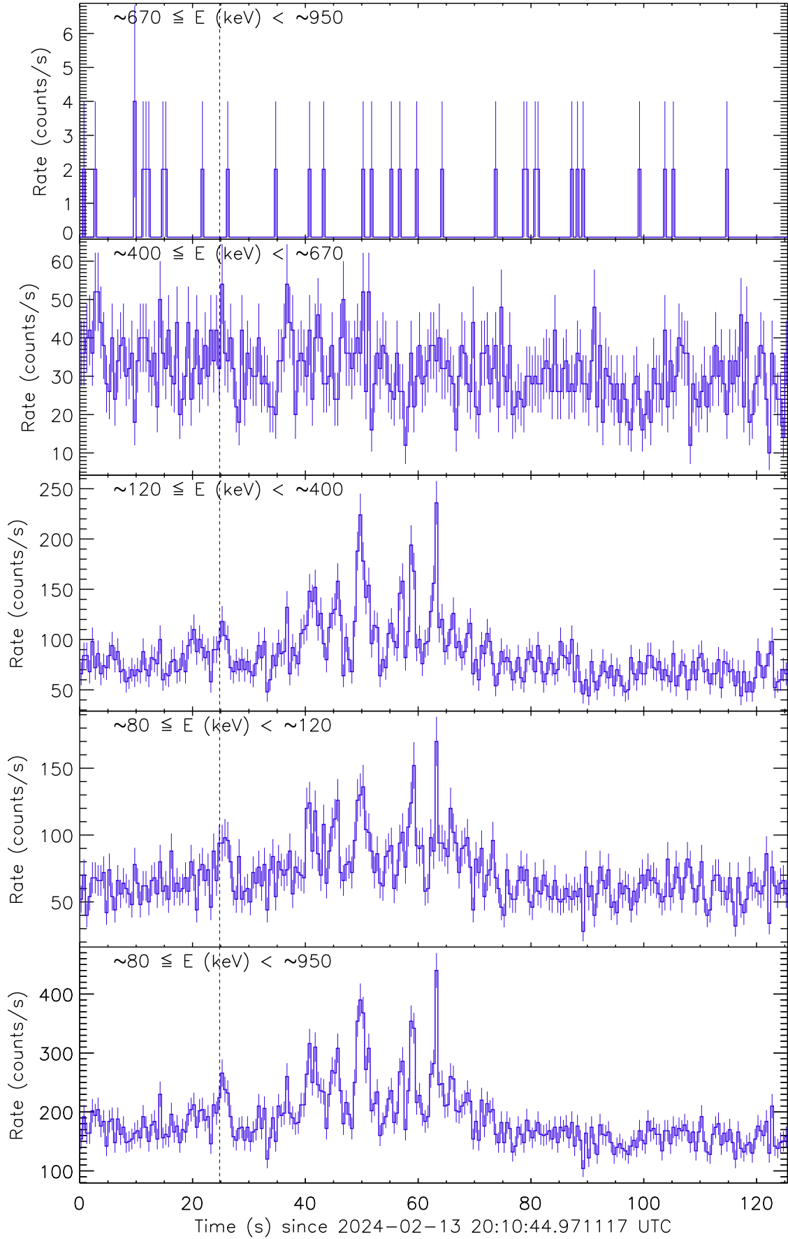
Figure 1: Raw count rate curve of GRB 240213A. The vertical dashed line marks the trigger time by Fermi/GBM.
