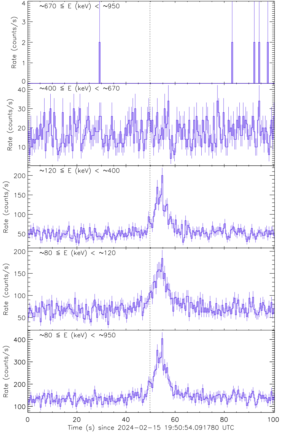
Figure 1: Raw count rate curve of GRB 240215B. The vertical dashed line marks the trigger time by Fermi/GBM.
