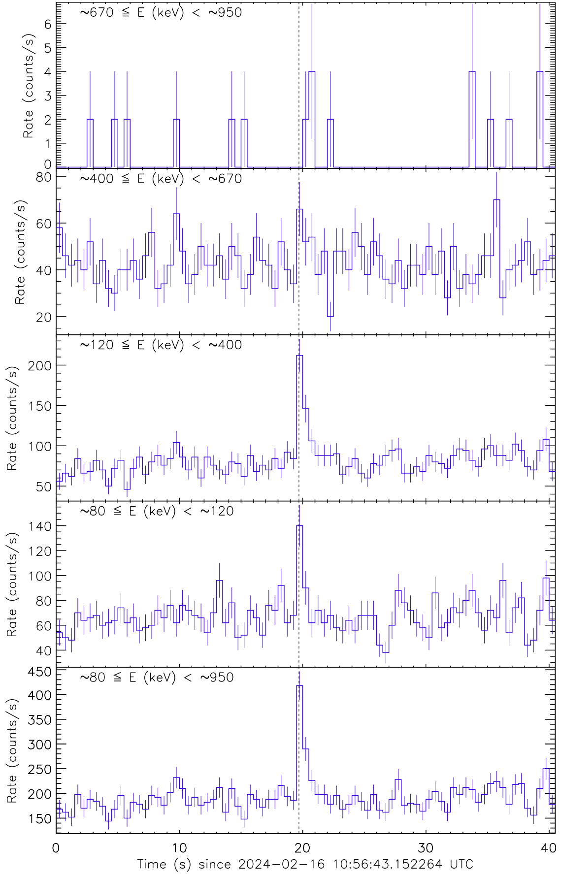
Figure 1: Raw count rate curve of GRB 240216A. The vertical dashed line marks the trigger time by Fermi/GBM.
