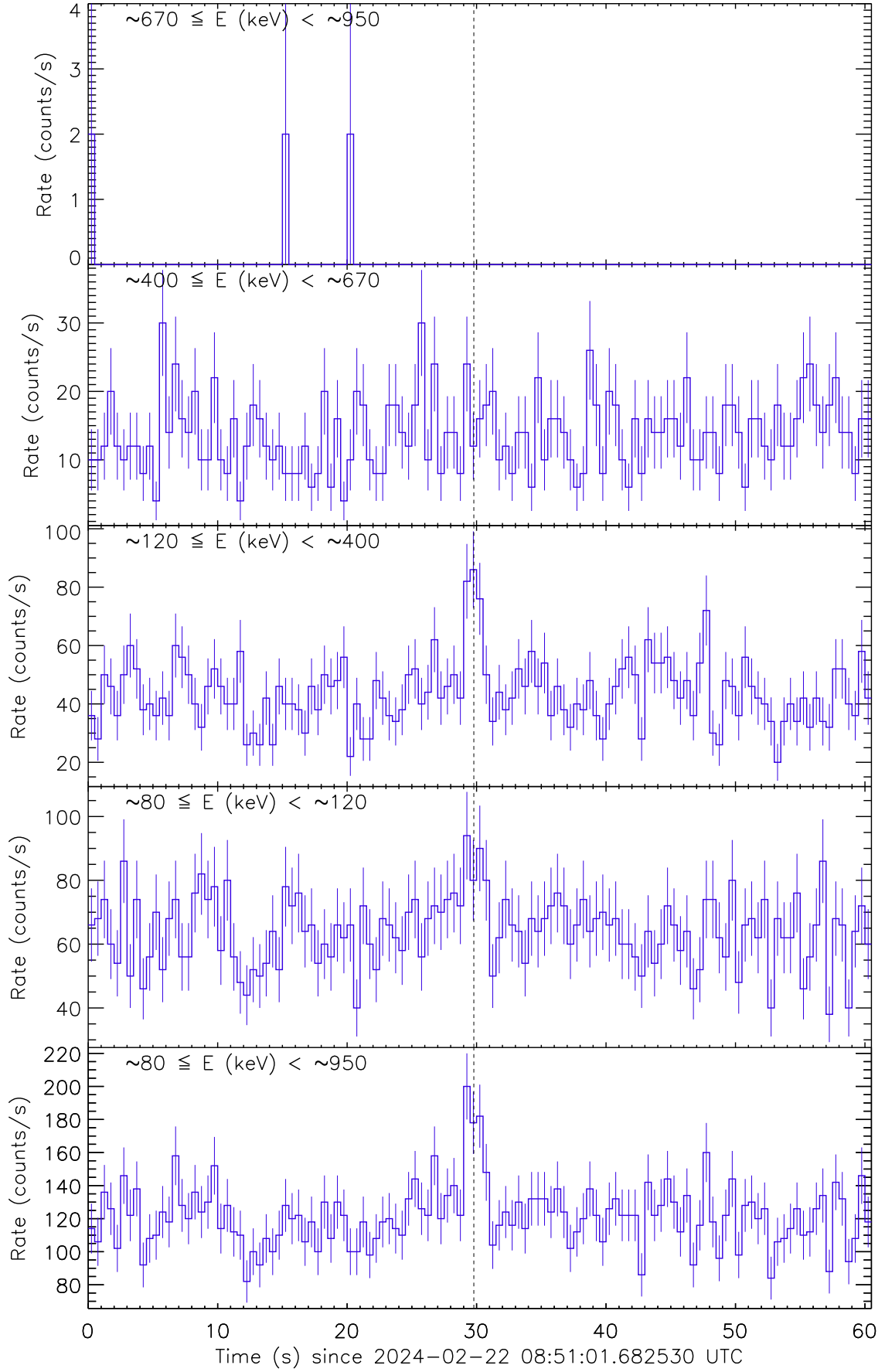
Figure 1: Raw count rate curve of GRB 240222A. The vertical dashed line marks the trigger time by Fermi/GBM.
