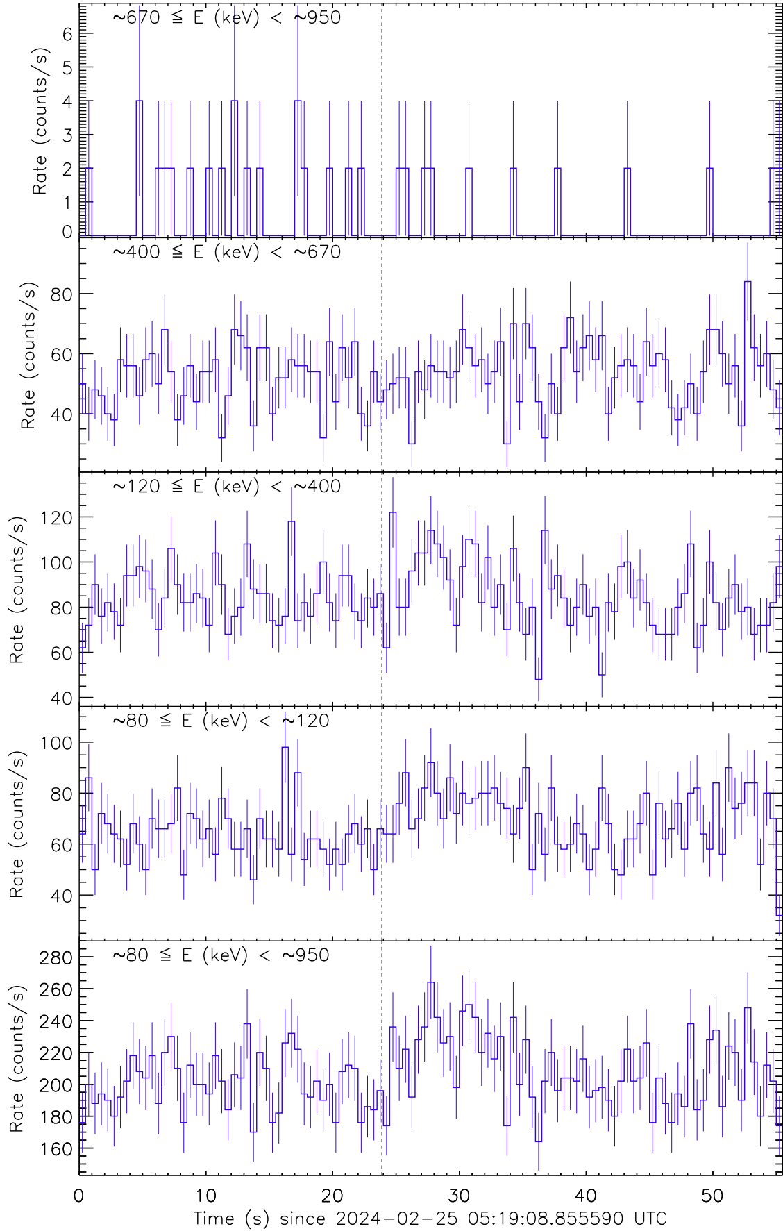
Figure 1: Raw count rate curve of GRB 240225C. The vertical dashed line marks the trigger time by CALET/CGBM.
