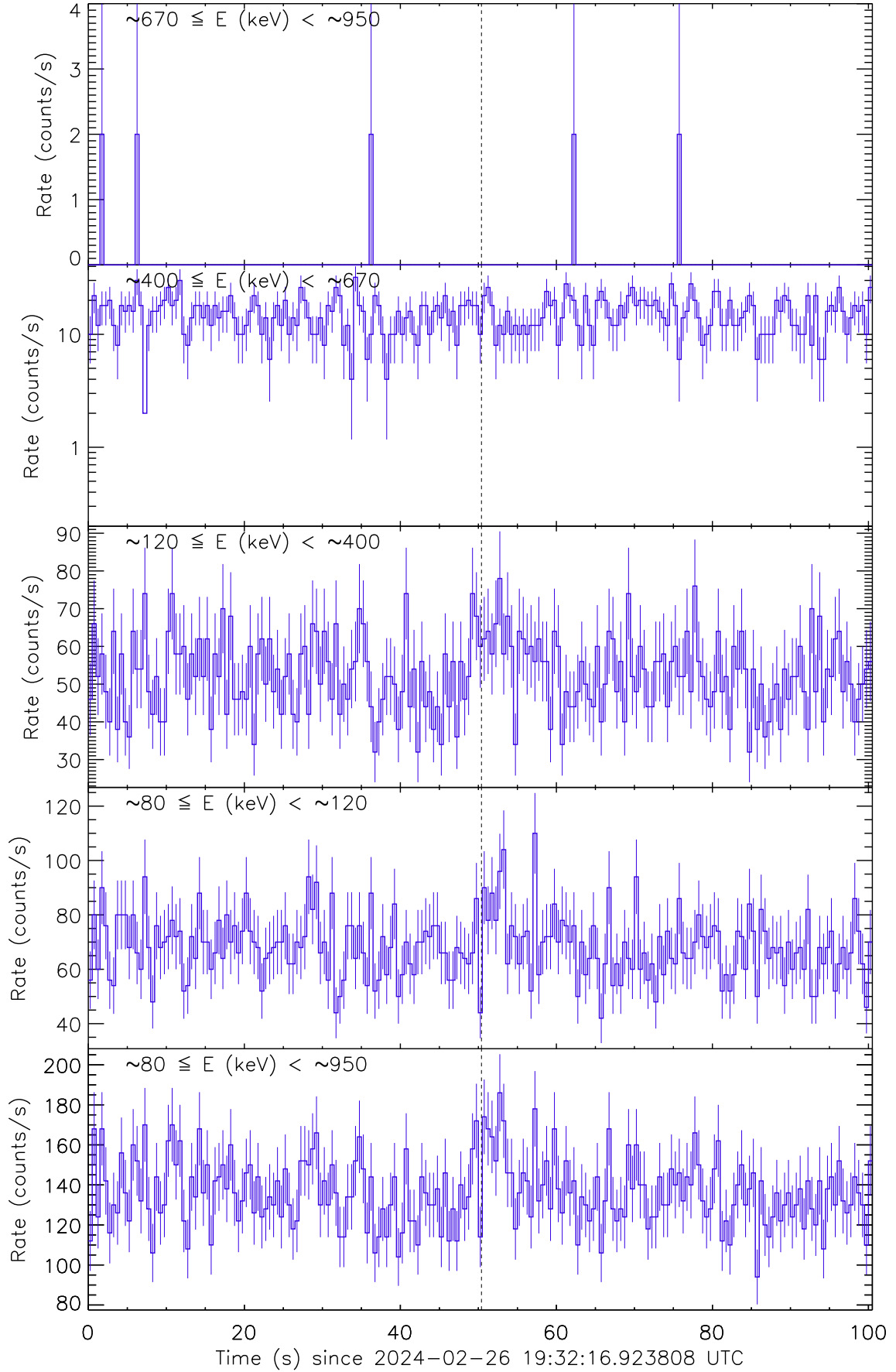
Figure 1: Raw count rate curve of GRB 240226A. The vertical dashed line marks the trigger time by Fermi/GBM.
