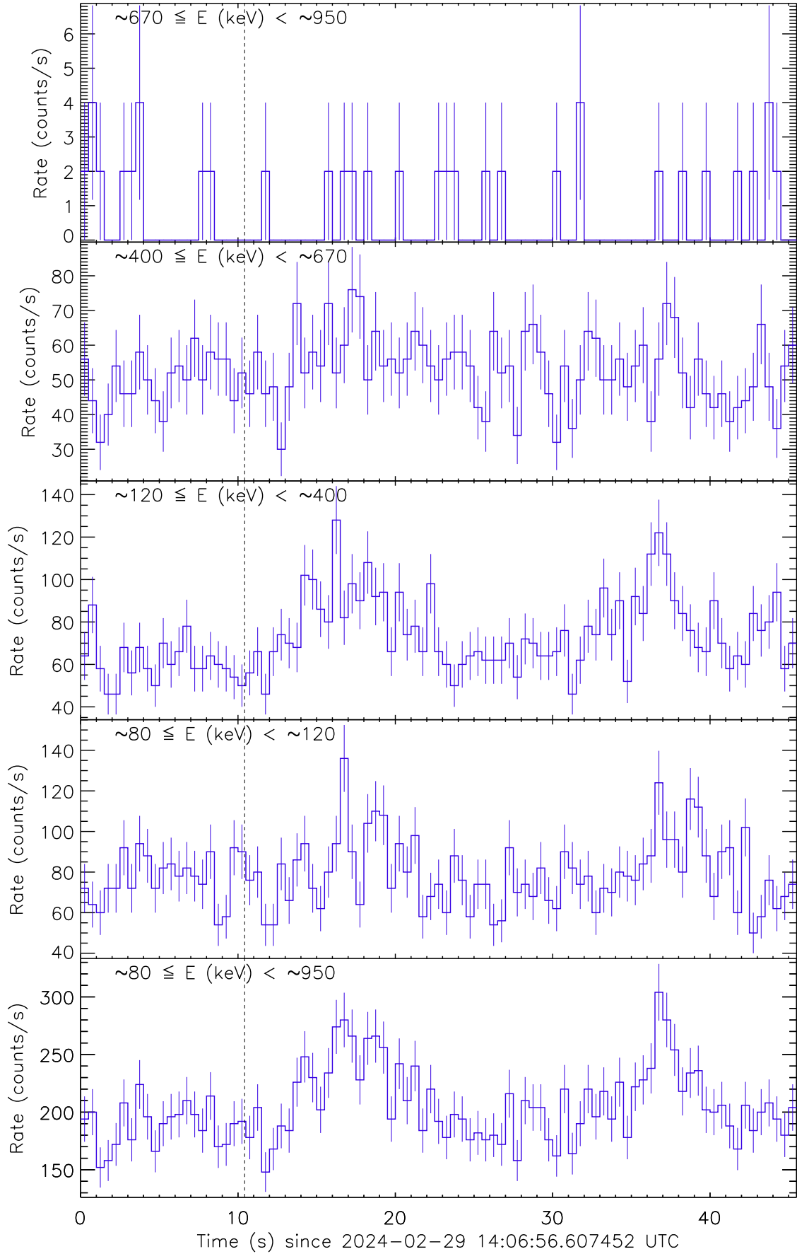
Figure 1: Raw count rate curve of GRB 240229A. The vertical dashed line marks the trigger time by Fermi/GBM.
