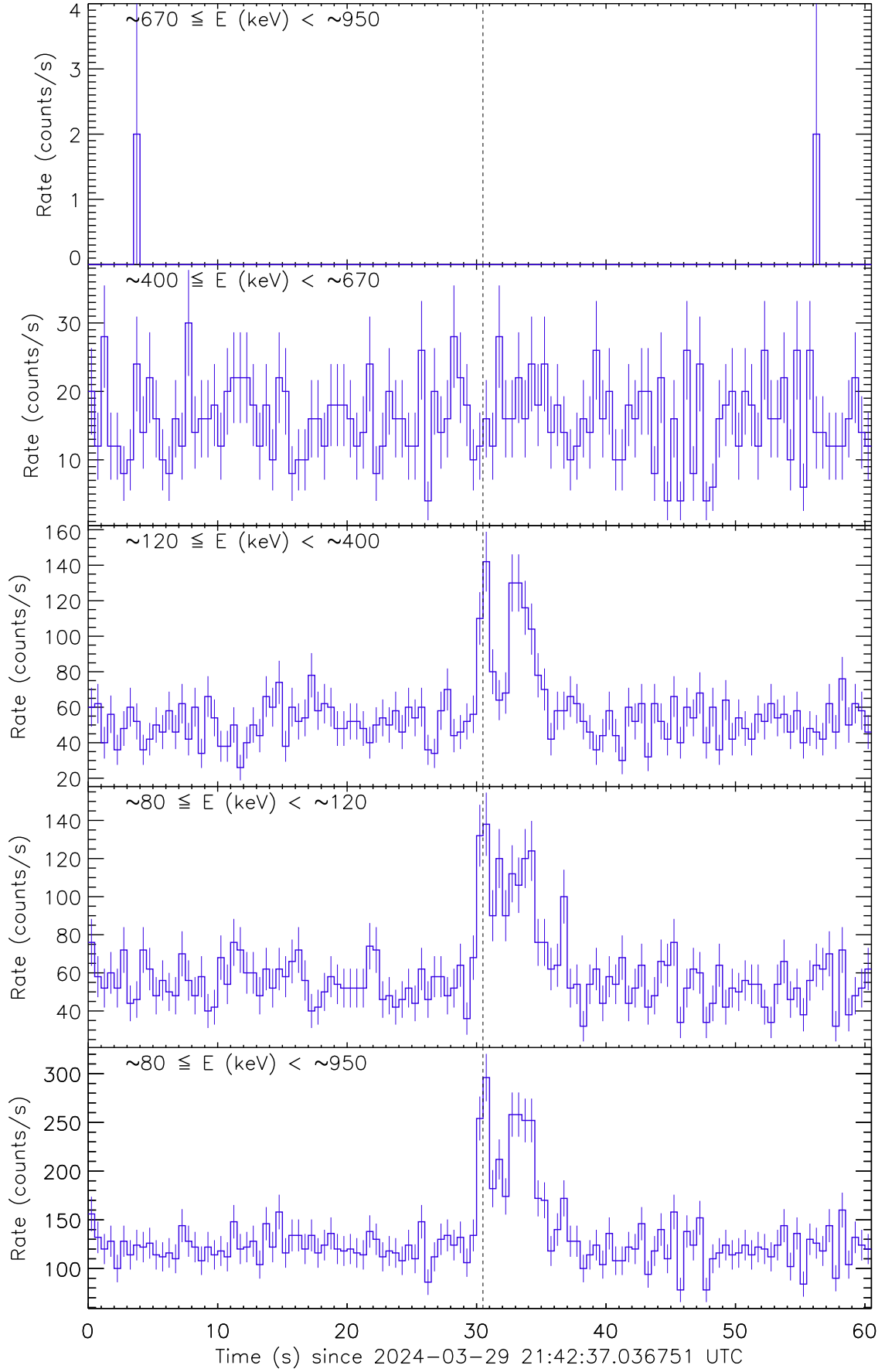
Figure 1: Raw count rate curve of GRB 240329A. The vertical dashed line marks the trigger time by Fermi/GBM.
