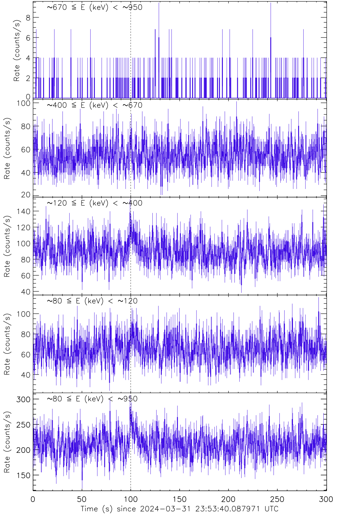
Figure 1: Raw count rate curve of GRB 240331A. The vertical dashed line marks the trigger time by Fermi/GBM.
