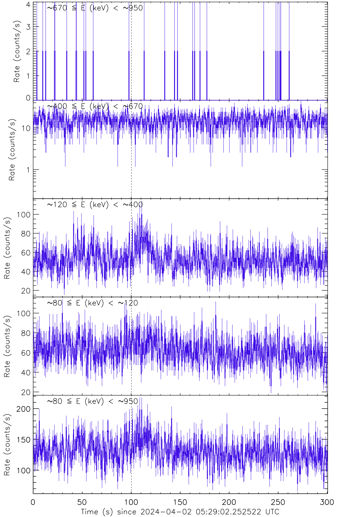
Figure 1: Raw count rate curve of GRB 240402C. The vertical dashed line marks the trigger time by CALET/CGBM.
