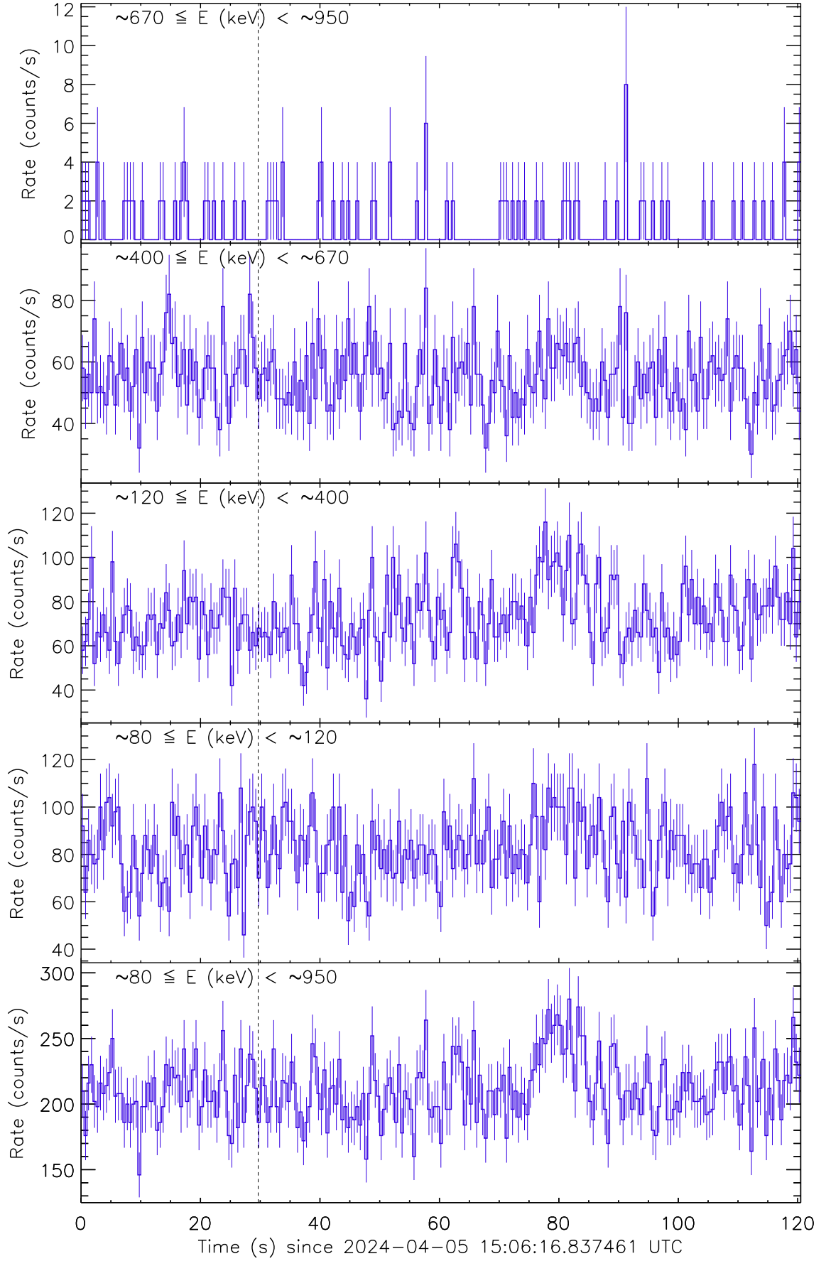
Figure 1: Raw count rate curve of GRB 240405A. The vertical dashed line marks the trigger time by Fermi/GBM.
