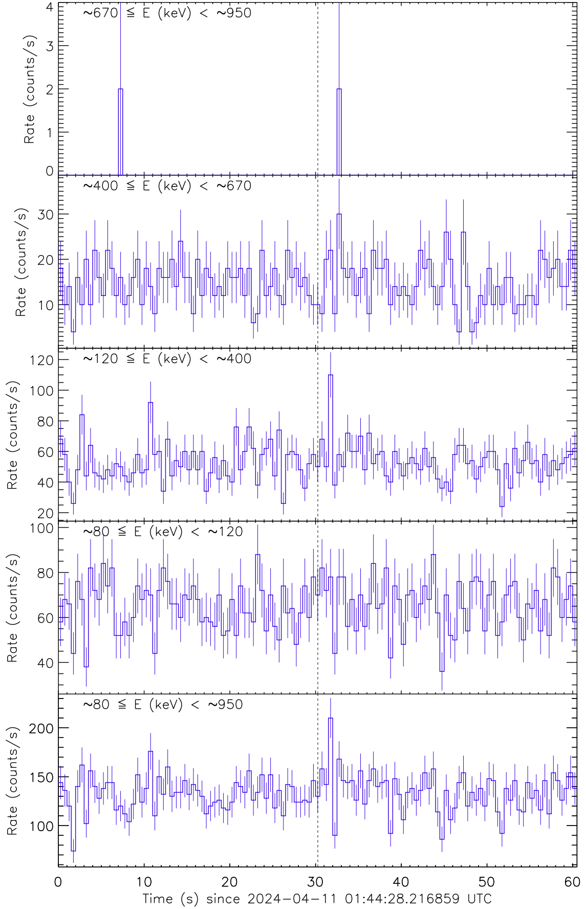
Figure 1: Raw count rate curve of GRB 240411A. The vertical dashed line marks the trigger time by Fermi/GBM.
