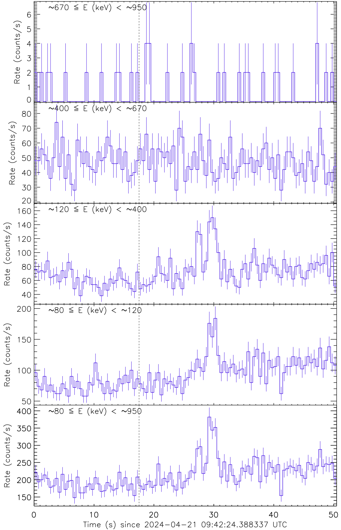
Figure 1: Raw count rate curve of GRB 240421B. The vertical dashed line marks the trigger time by Fermi/GBM.
