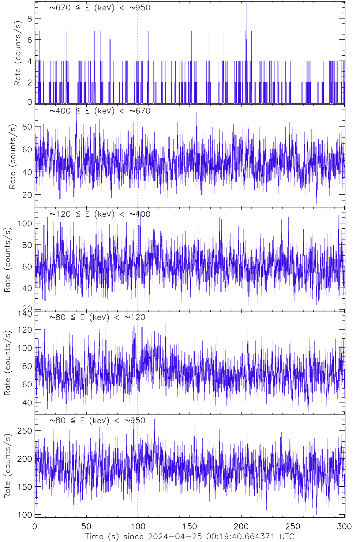
Figure 1: Raw count rate curve of GRB 240425A. The vertical dashed line marks the trigger time by Fermi/GBM.
