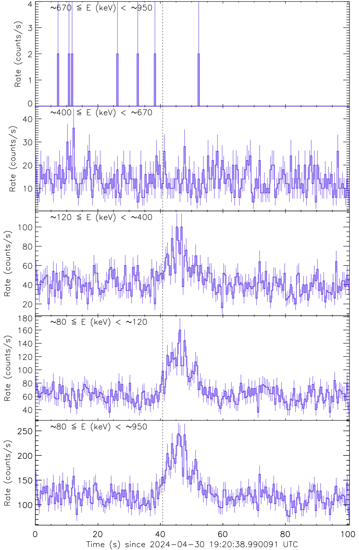
Figure 1: Raw count rate curve of GRB 240430A. The vertical dashed line marks the trigger time by Fermi/GBM.
