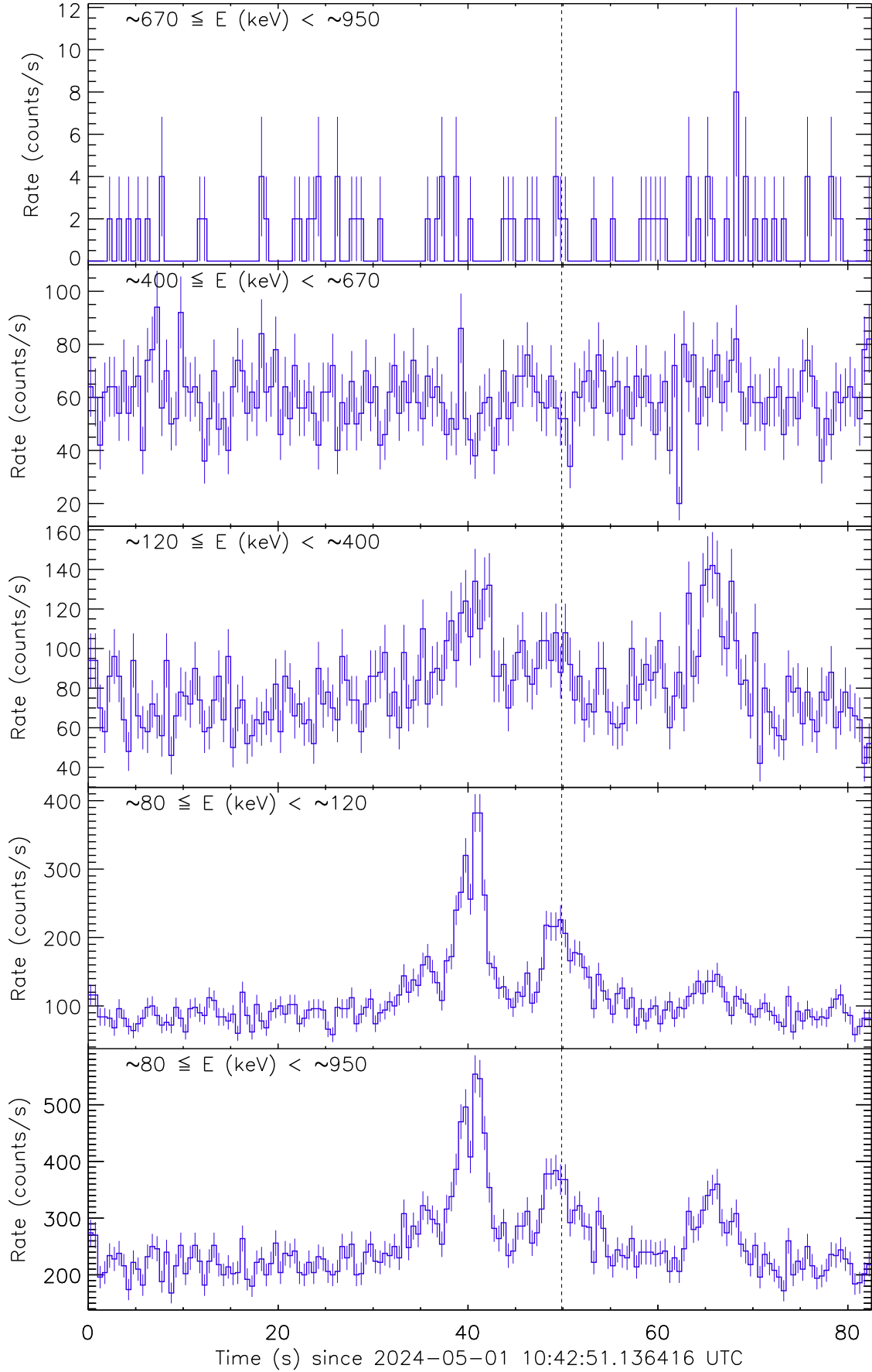
Figure 1: Raw count rate curve of GRB 240501B. The vertical dashed line marks the trigger time by AstroSat/CZTI.
