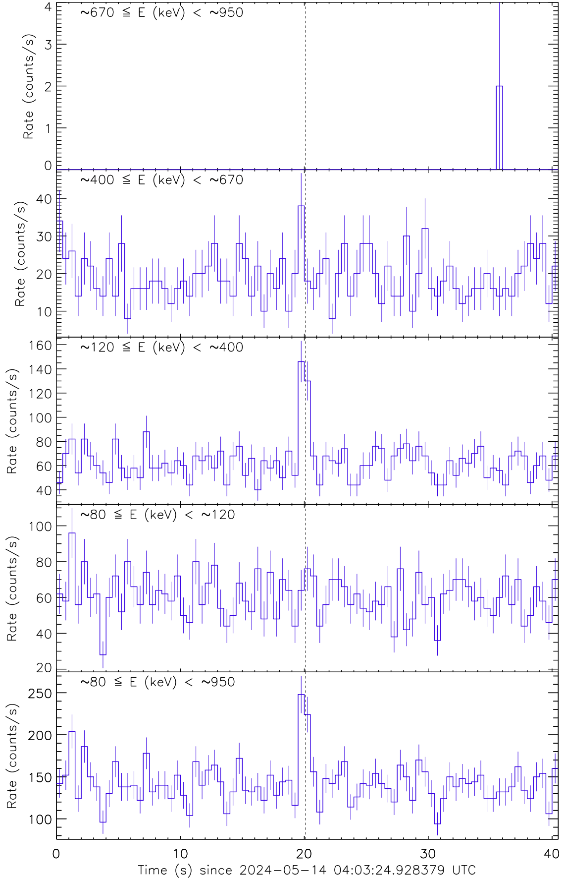
Figure 1: Raw count rate curve of GRB 240514B. The vertical dashed line marks the trigger time by Fermi/GBM.
