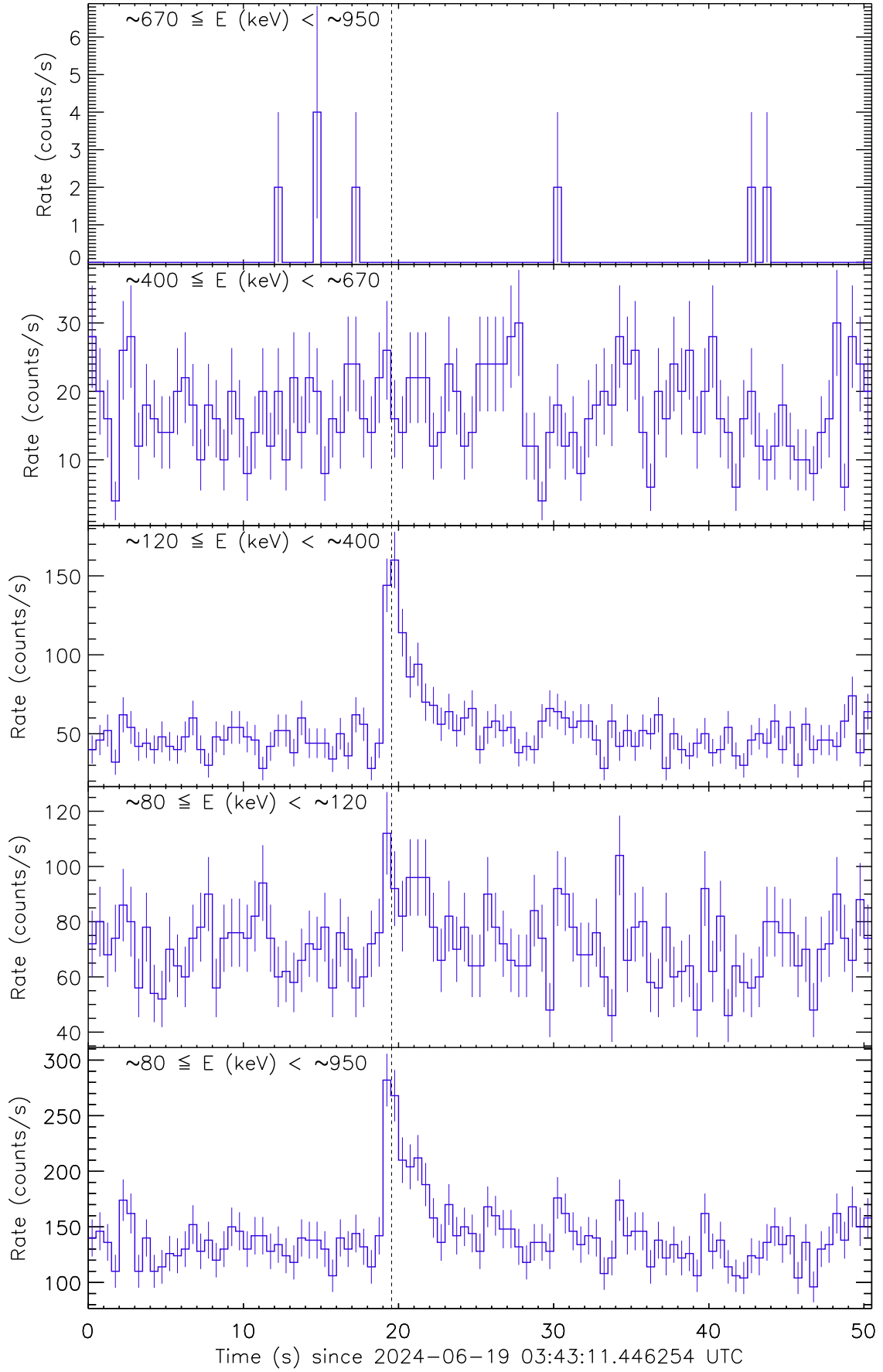
Figure 1: Raw count rate curve of GRB 240619A. The vertical dashed line marks the trigger time by Fermi/GBM.
