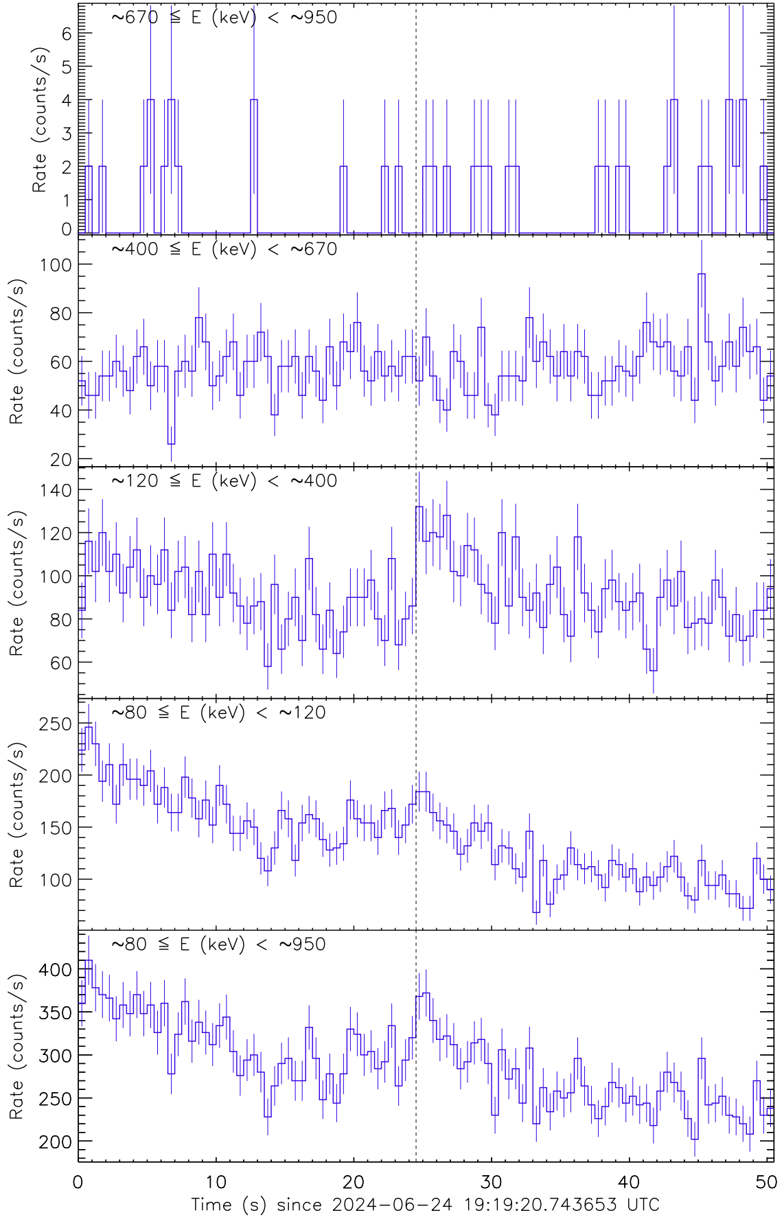
Figure 1: Raw count rate curve of GRB 240624B. The vertical dashed line marks the trigger time by Fermi/GBM.
