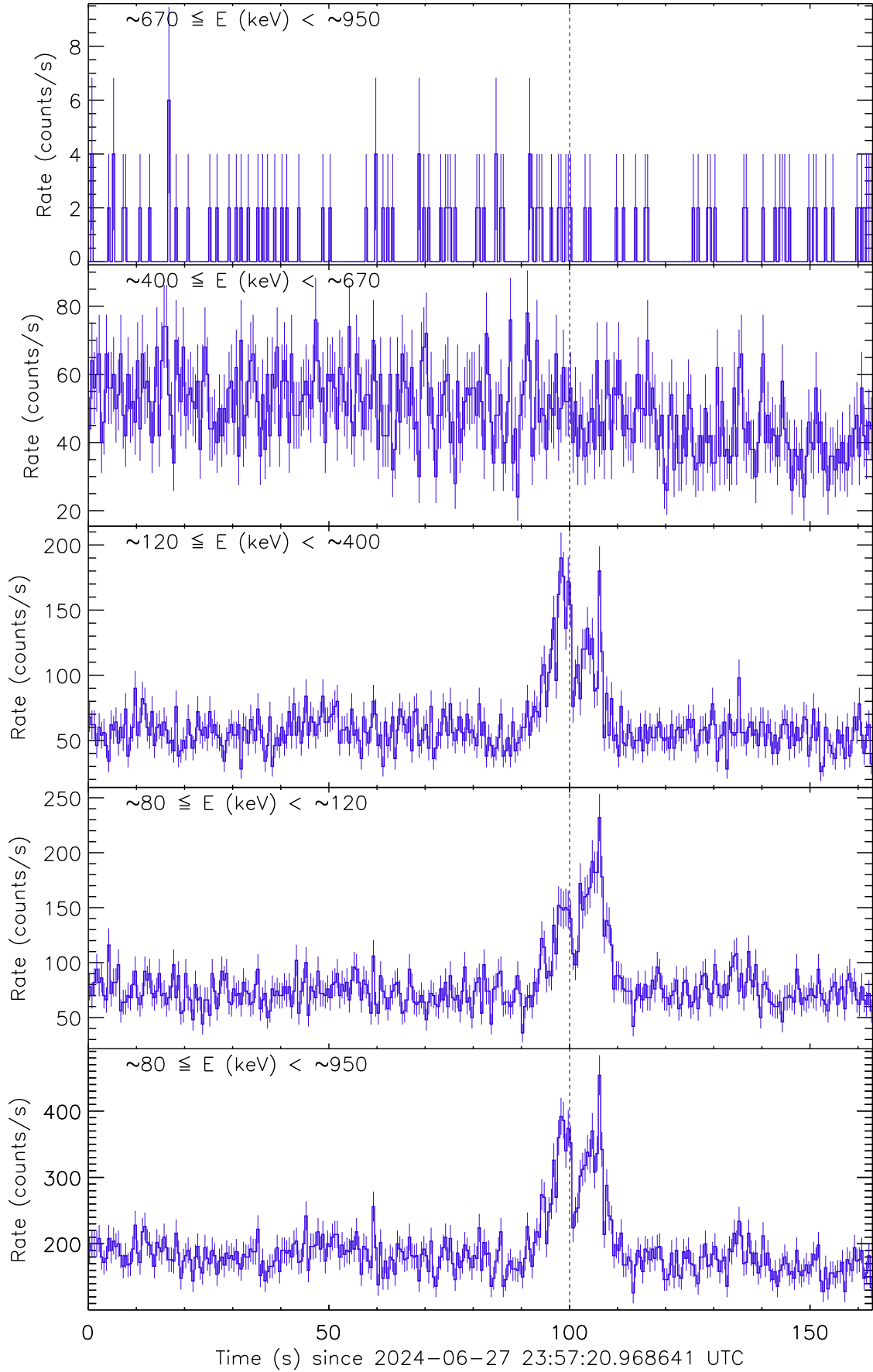
Figure 1: Raw count rate curve of GRB 240627A. The vertical dashed line marks the trigger time by AstroSat/CZTI.
