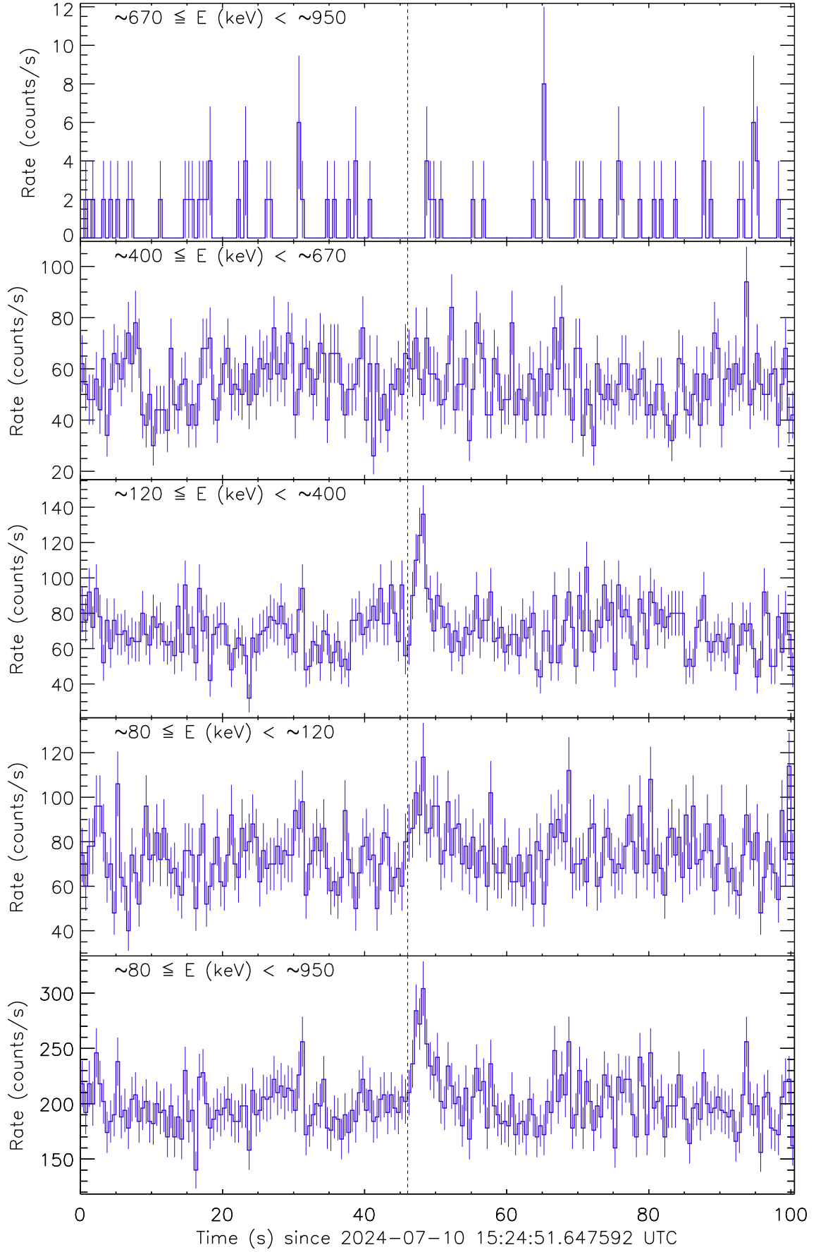
Figure 1: Raw count rate curve of GRB 240710B. The vertical dashed line marks the trigger time by Fermi/GBM.
