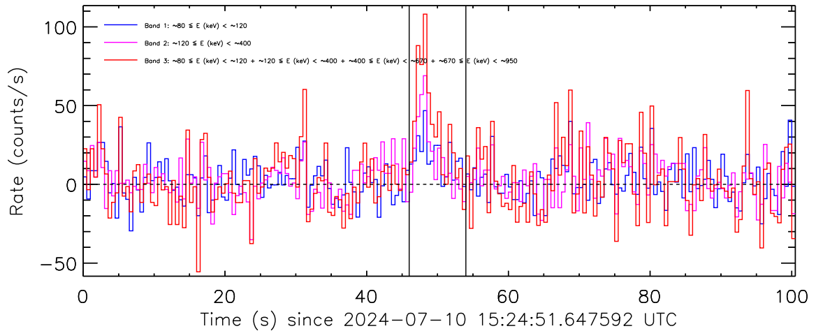
Figure 3: Background-subtracted count rate curve.
