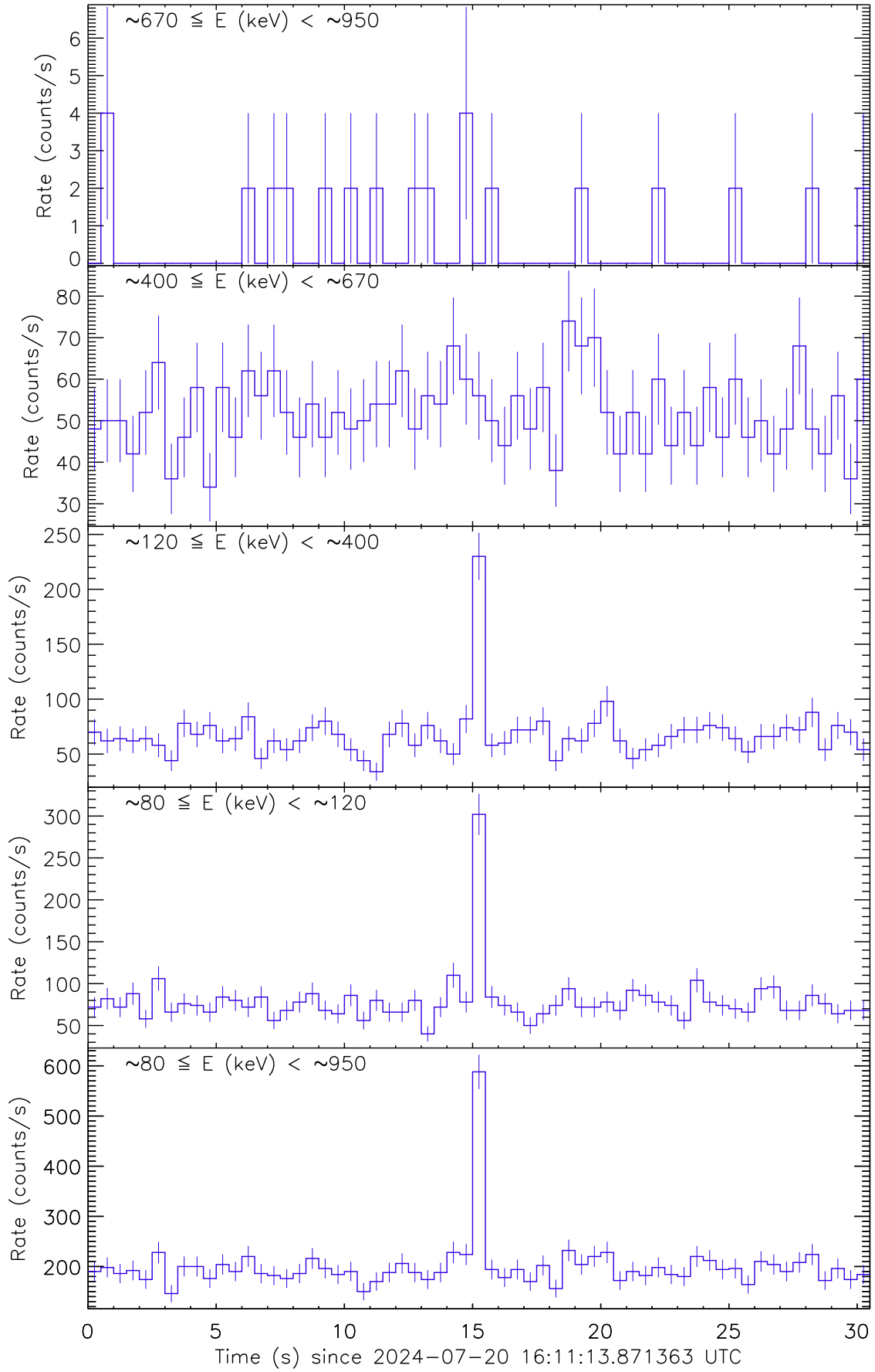
Figure 1: Raw count rate curve of GRB 240720B.
