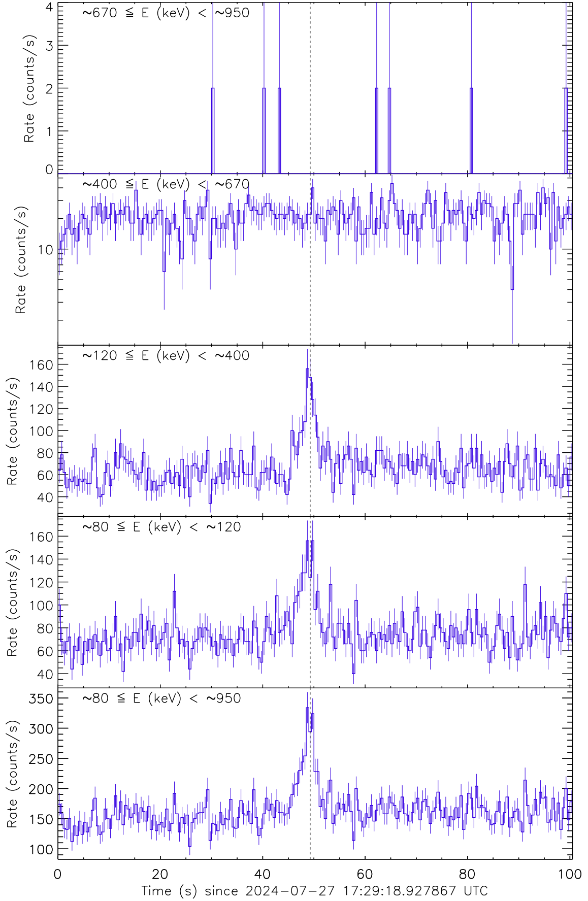
Figure 1: Raw count rate curve of GRB 240727C. The vertical dashed line marks the trigger time by AstroSat/CZTI.
