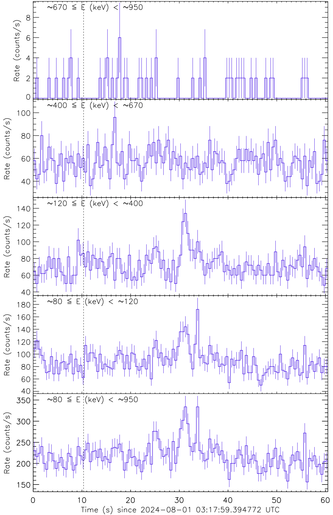
Figure 1: Raw count rate curve of GRB 240801A. The vertical dashed line marks the trigger time by Fermi/GBM.
