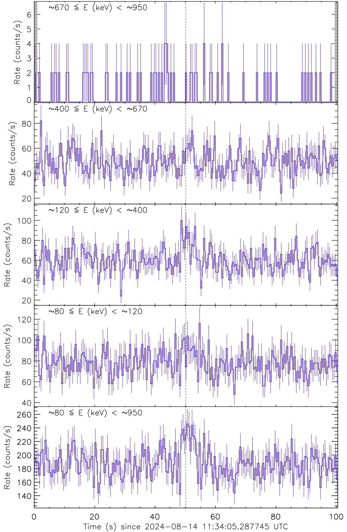
Figure 1: Raw count rate curve of GRB 240814B. The vertical dashed line marks the trigger time by Fermi/GBM.
