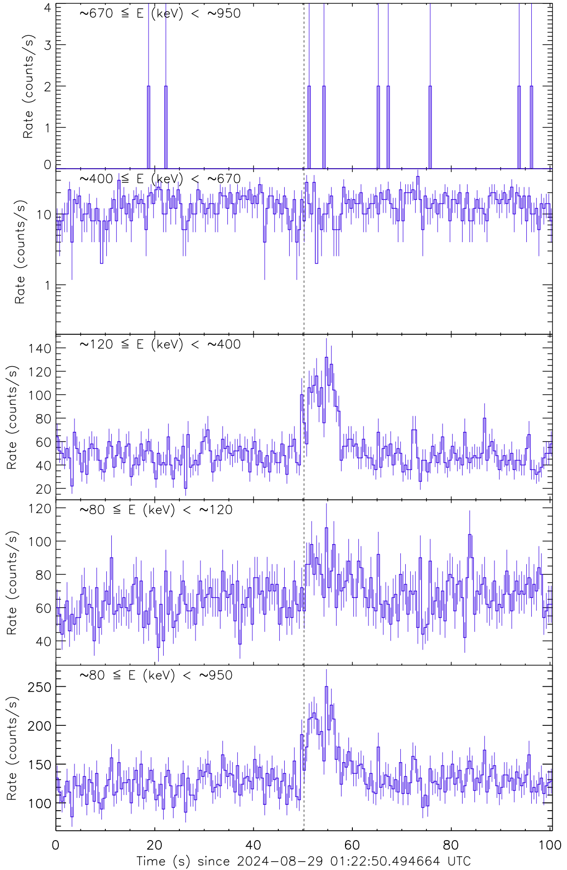
Figure 1: Raw count rate curve of GRB 240829B. The vertical dashed line marks the trigger time by Fermi/GBM.
