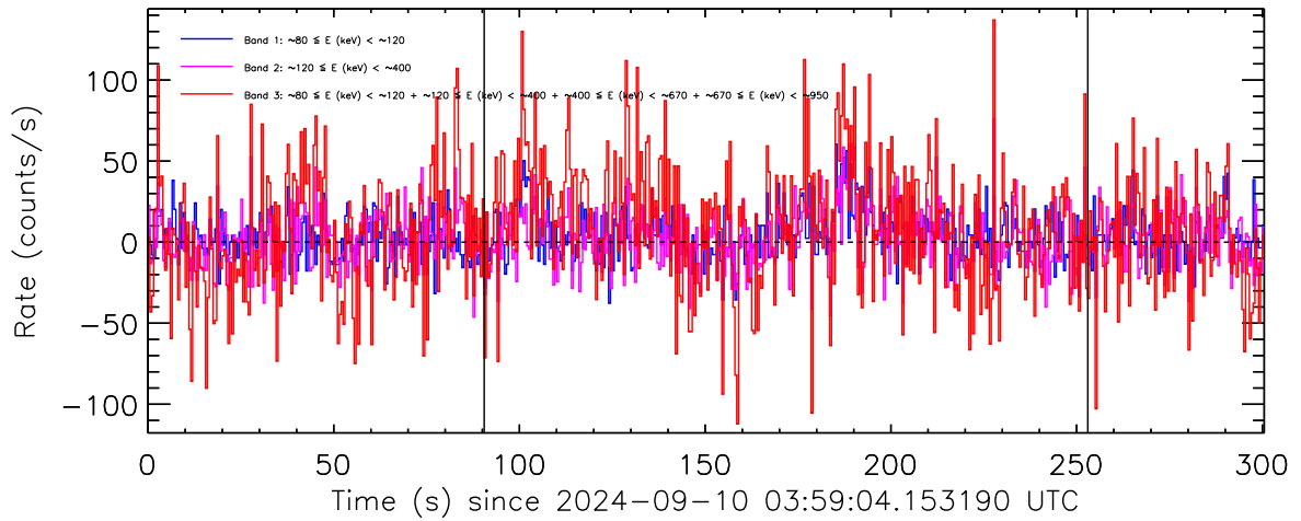
Figure 3: Background-subtracted count rate curve.
