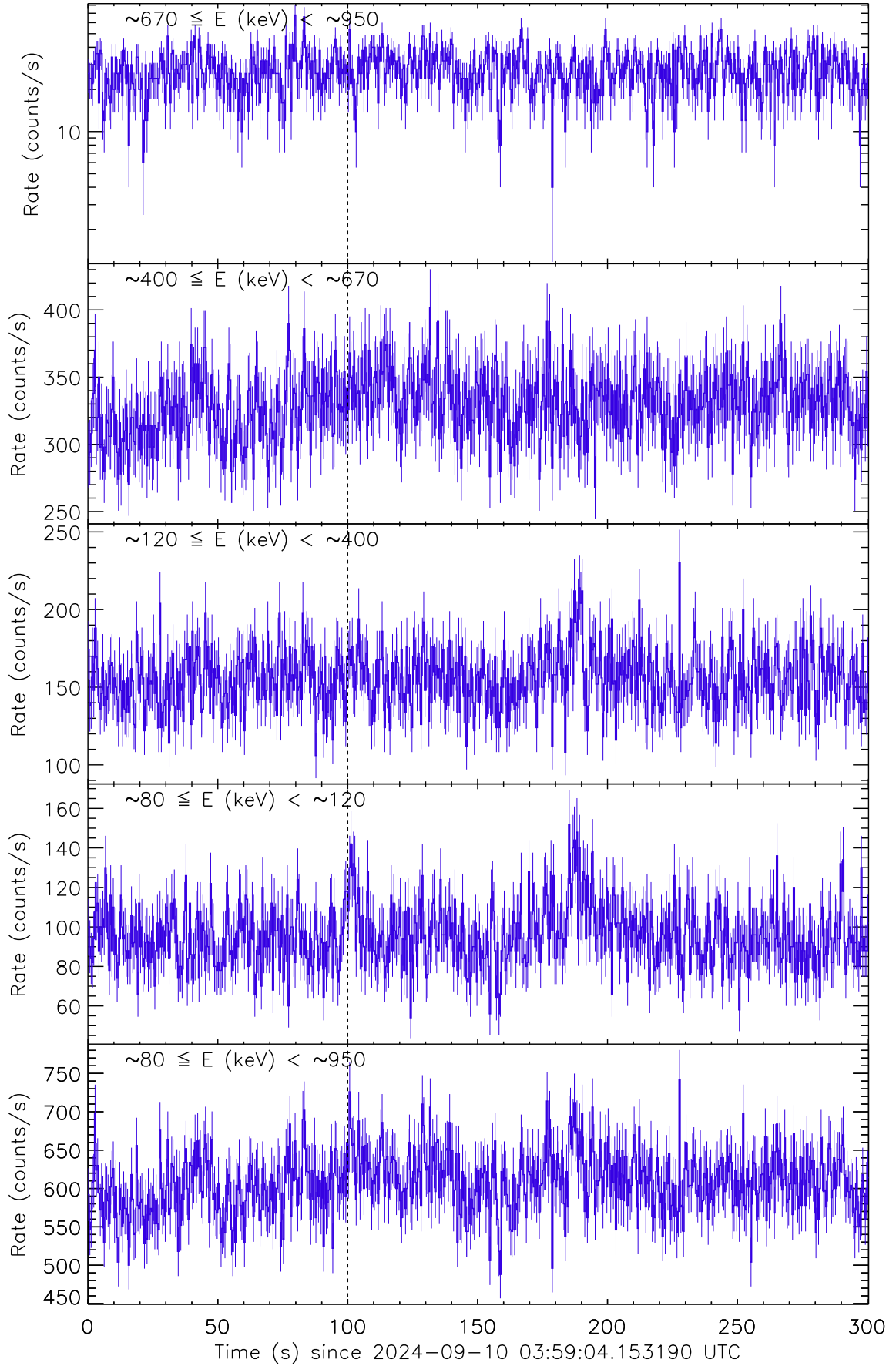
Figure 1: Raw count rate curve of GRB 240910A. The vertical dashed line marks the trigger time by Fermi/GBM.
