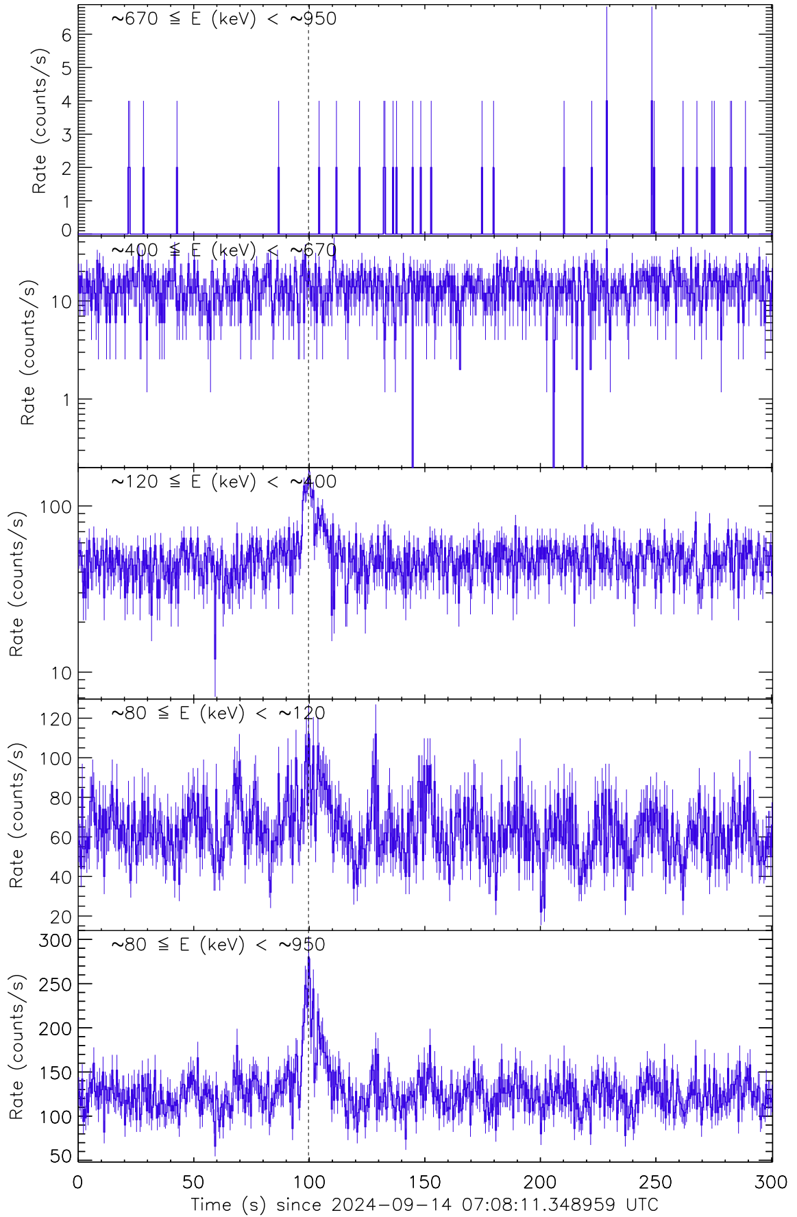
Figure 1: Raw count rate curve of GRB 240914B. The vertical dashed line marks the trigger time by Fermi/GBM.
