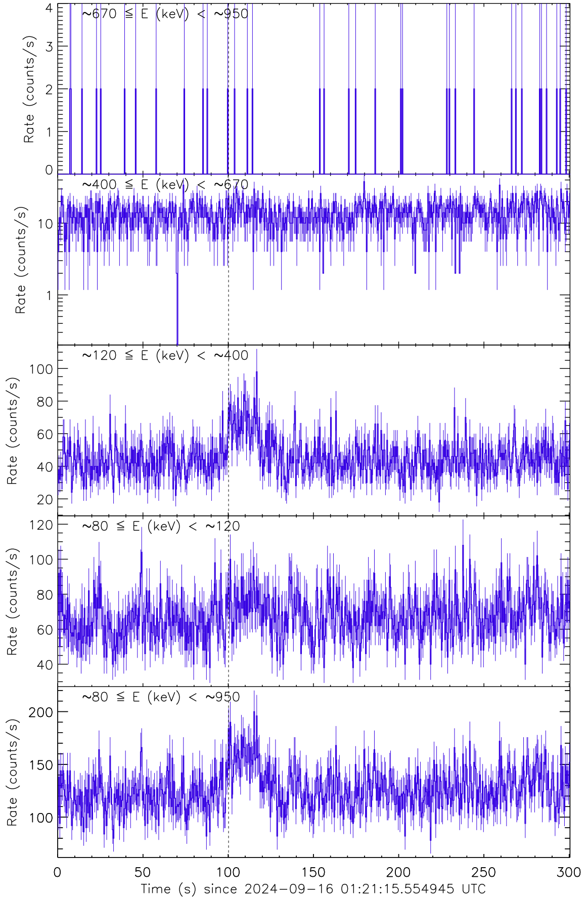
Figure 1: Raw count rate curve of GRB 240916A. The vertical dashed line marks the trigger time by Fermi/GBM.
