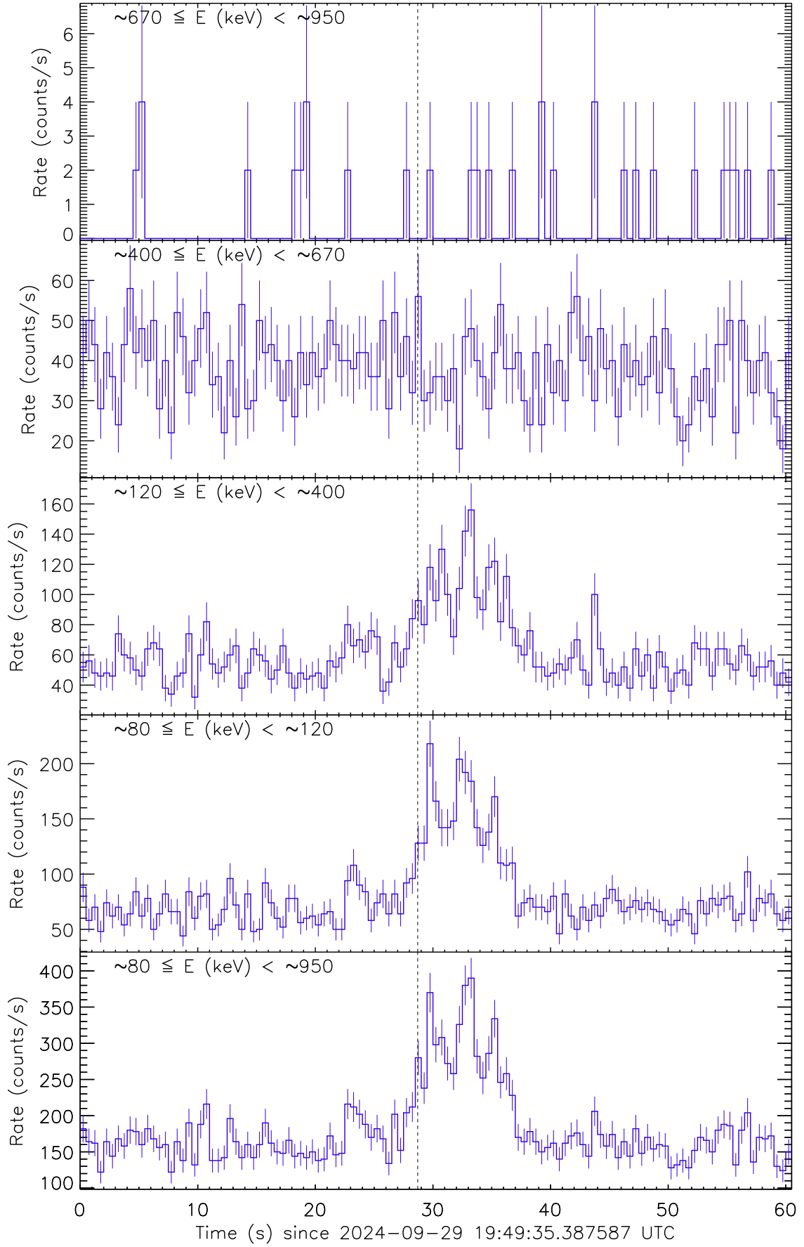
Figure 1: Raw count rate curve of GRB 240929A. The vertical dashed line marks the trigger time by Fermi/GBM.
