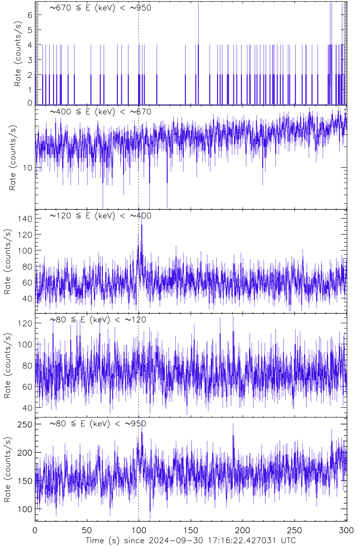
Figure 1: Raw count rate curve of GRB 240930B. The vertical dashed line marks the trigger time by Fermi/GBM.
