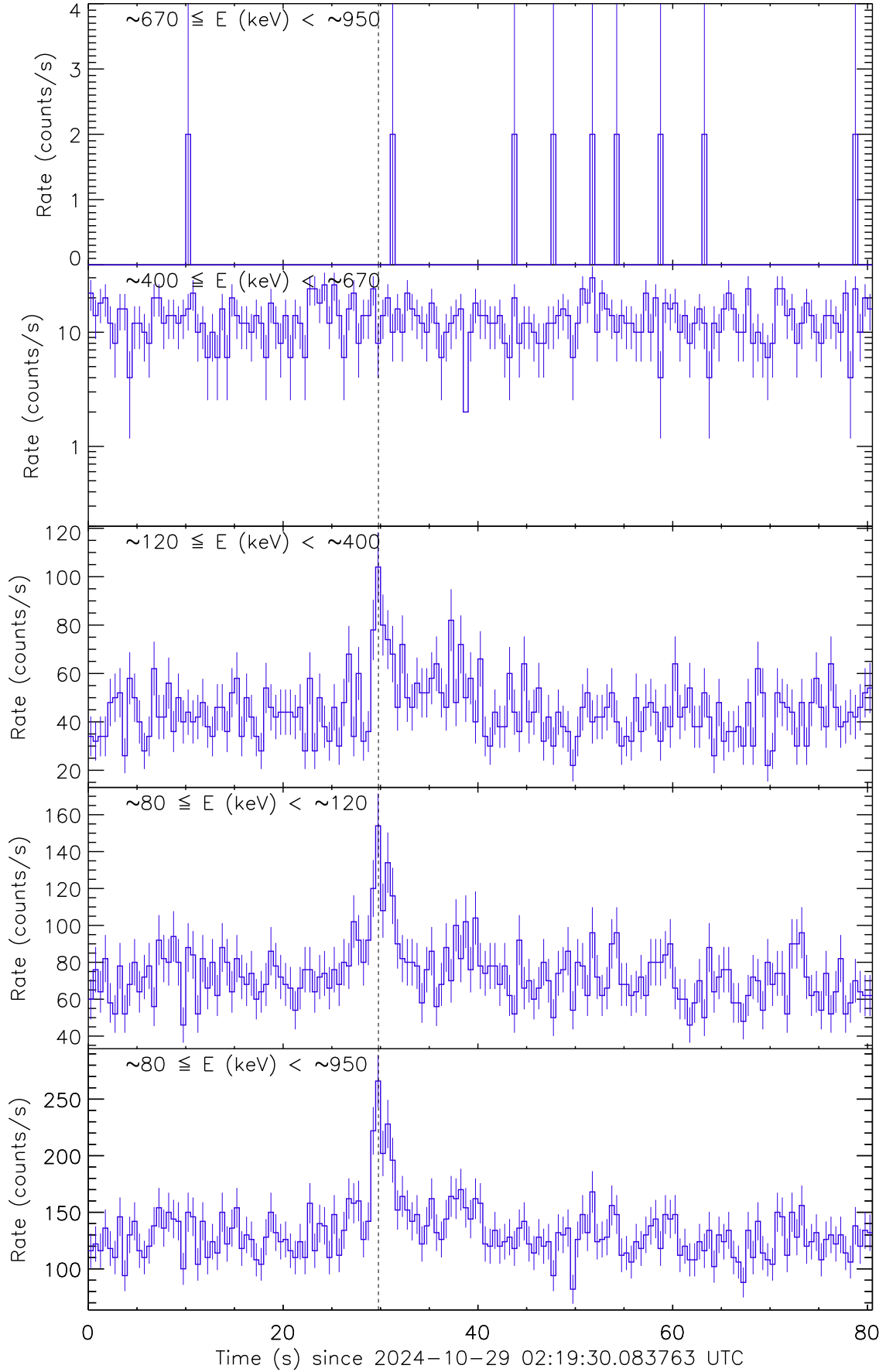
Figure 1: Raw count rate curve of GRB 241029A. The vertical dashed line marks the trigger time by Fermi/GBM.
