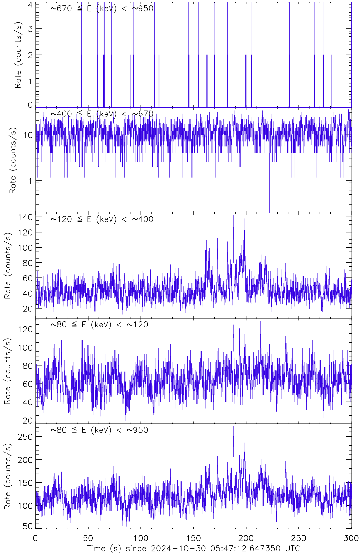
Figure 1: Raw count rate curve of GRB 241030A. The vertical dashed line marks the trigger time by Fermi/GBM.
