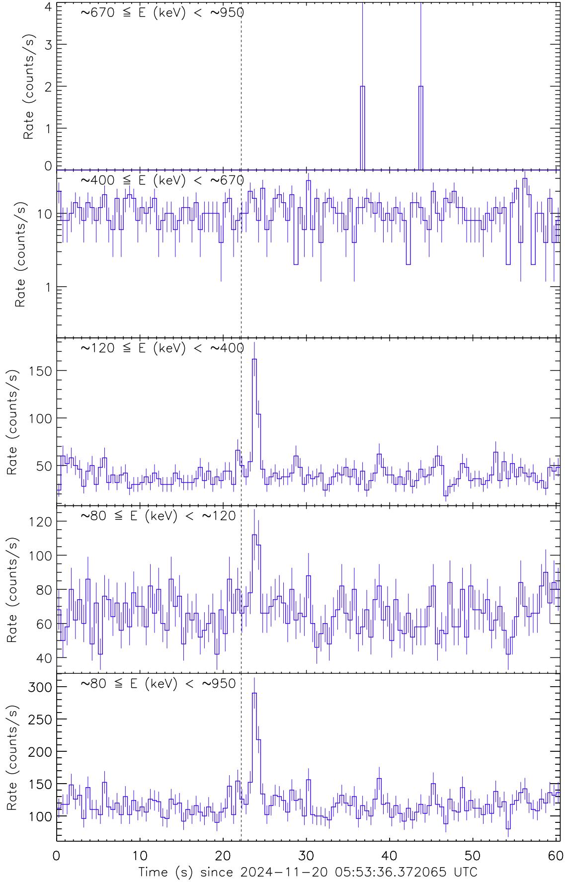
Figure 1: Raw count rate curve of GRB 241120A. The vertical dashed line marks the trigger time by Fermi/GBM.
