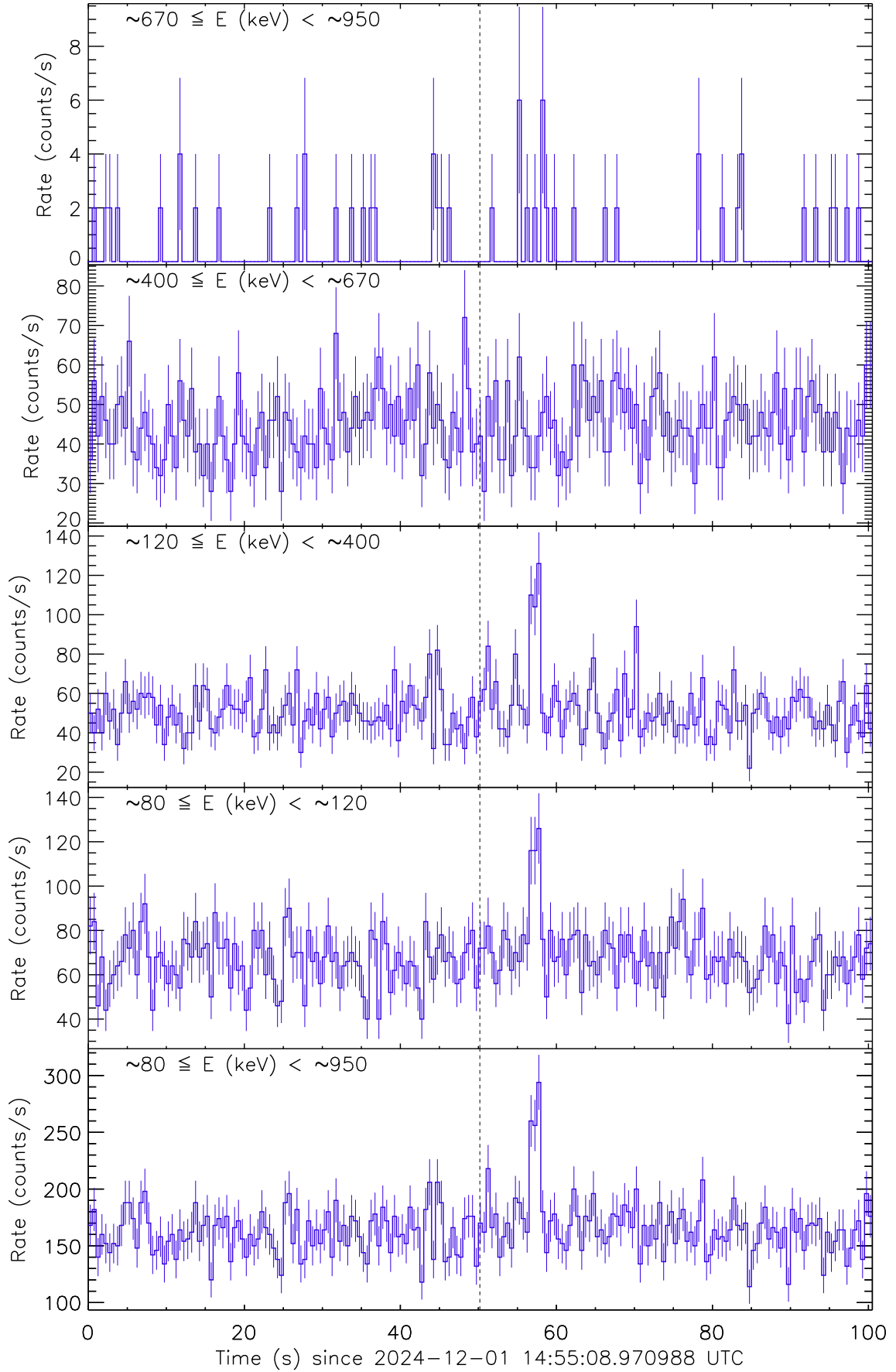
Figure 1: Raw count rate curve of GRB 241201A. The vertical dashed line marks the trigger time by Fermi/GBM.
