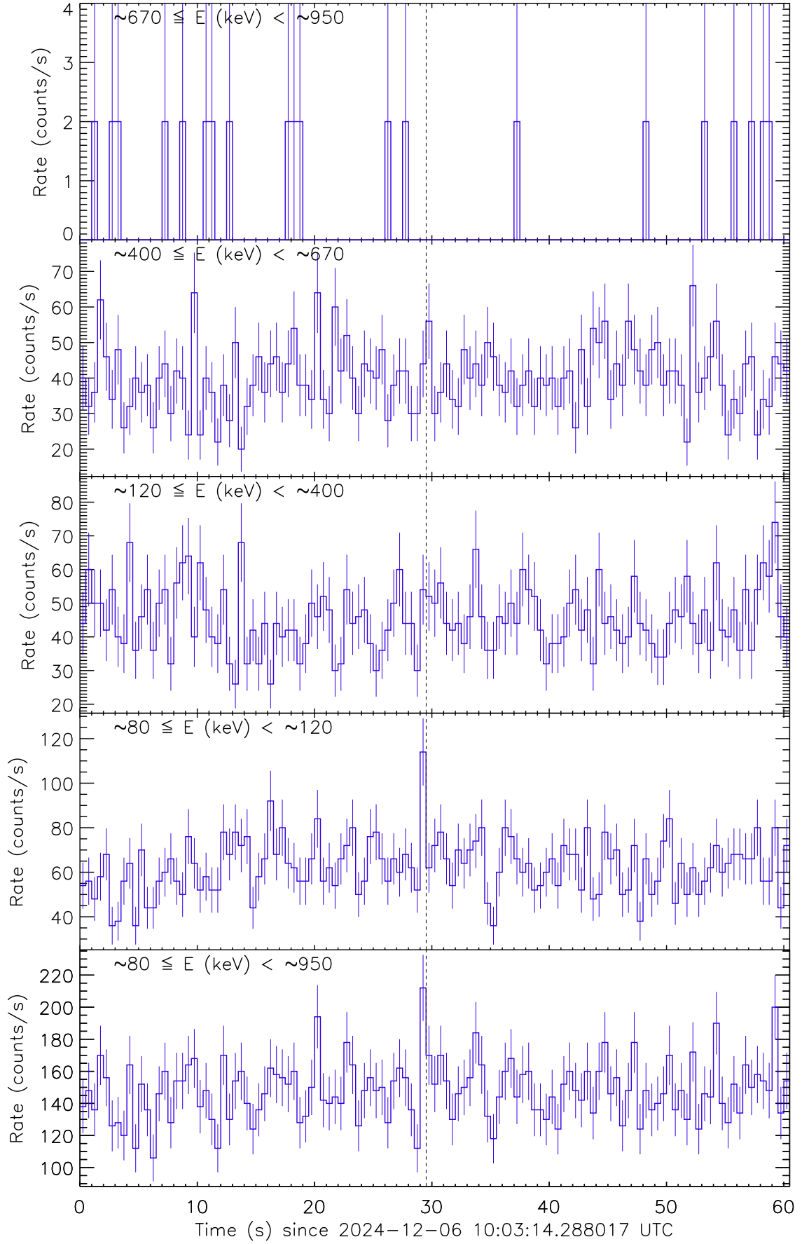
Figure 1: Raw count rate curve of GRB 241206C. The vertical dashed line marks the trigger time by SVOM/GRM.
