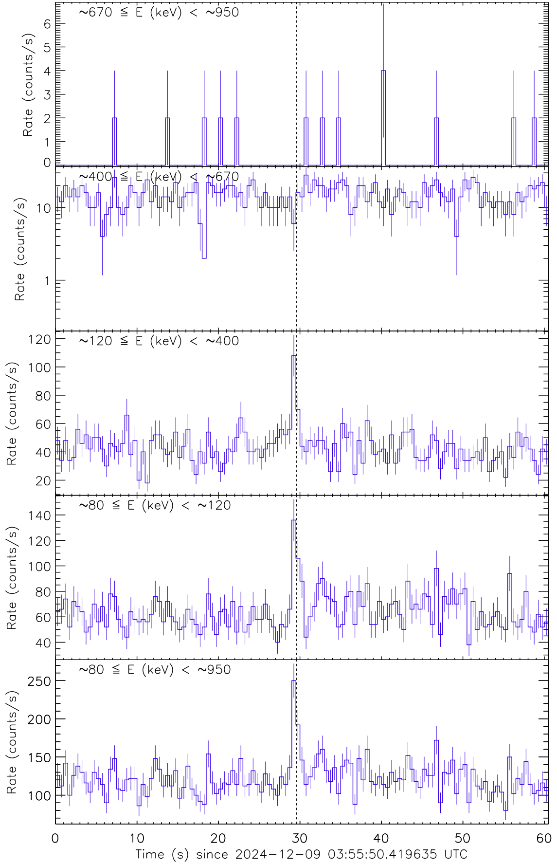
Figure 1: Raw count rate curve of GRB 241209B. The vertical dashed line marks the trigger time by SVOM/GRM.
