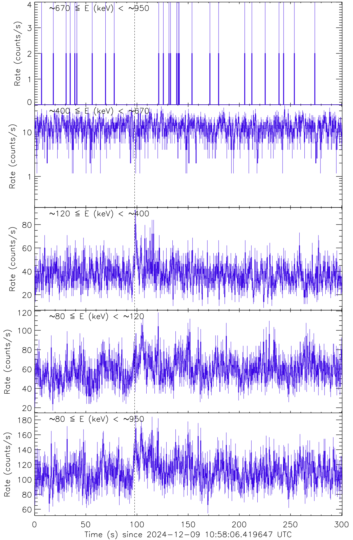
Figure 1: Raw count rate curve of GRB 241209D. The vertical dashed line marks the trigger time by Fermi/GBM.
