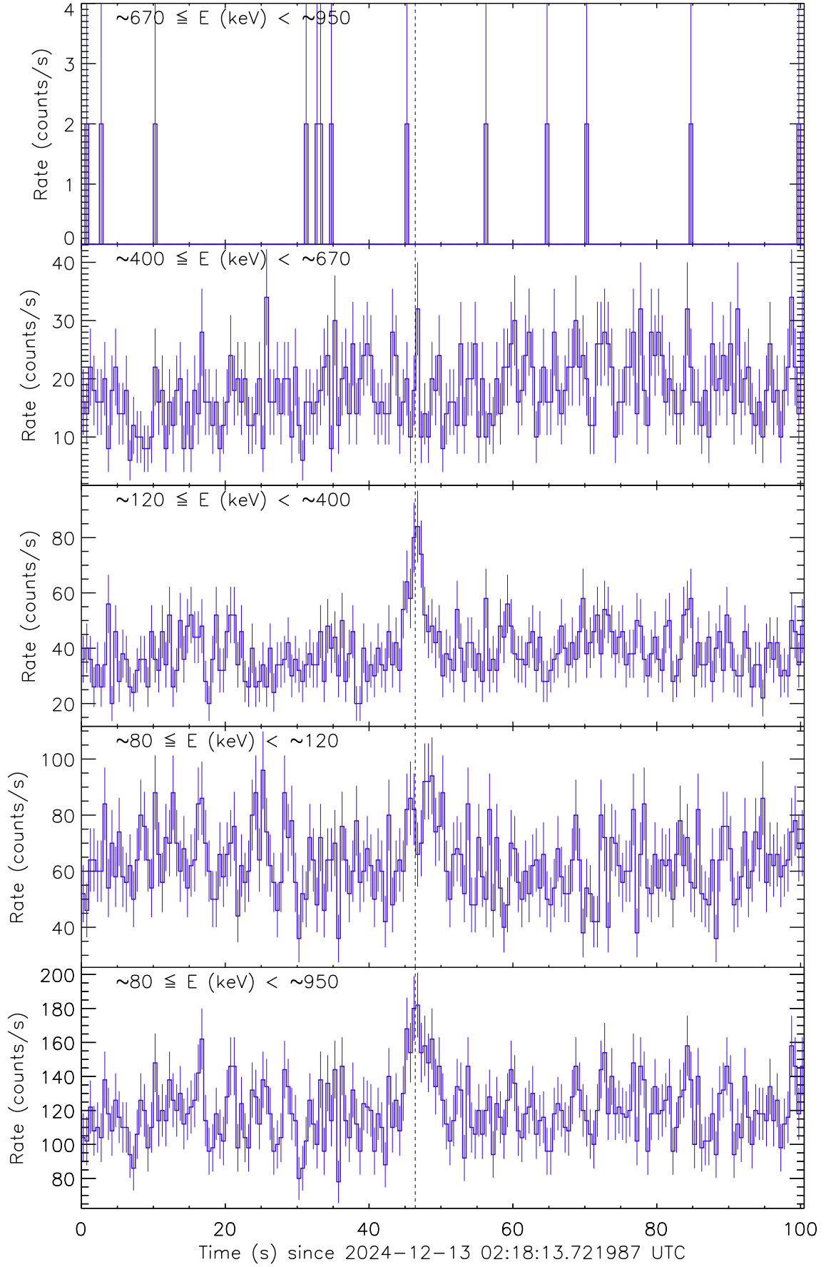
Figure 1: Raw count rate curve of GRB 241213A. The vertical dashed line marks the trigger time by Swift/BAT.
