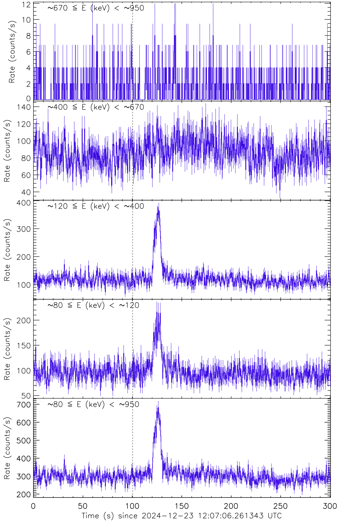
Figure 1: Raw count rate curve of GRB 241223A. The vertical dashed line marks the trigger time by Fermi/GBM.
