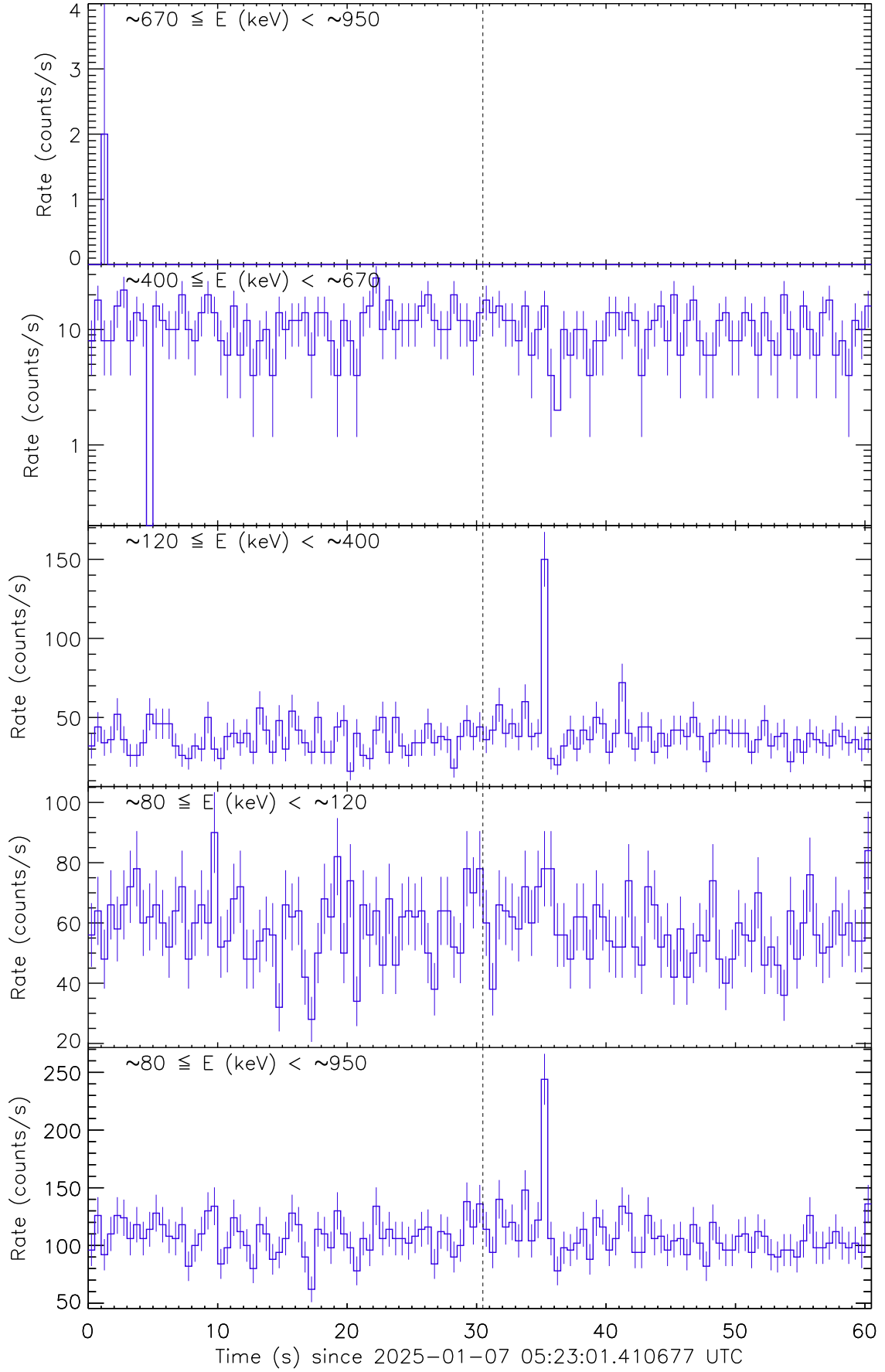
Figure 1: Raw count rate curve of GRB 250107D. The vertical dashed line marks the trigger time by Wind/Konus.
