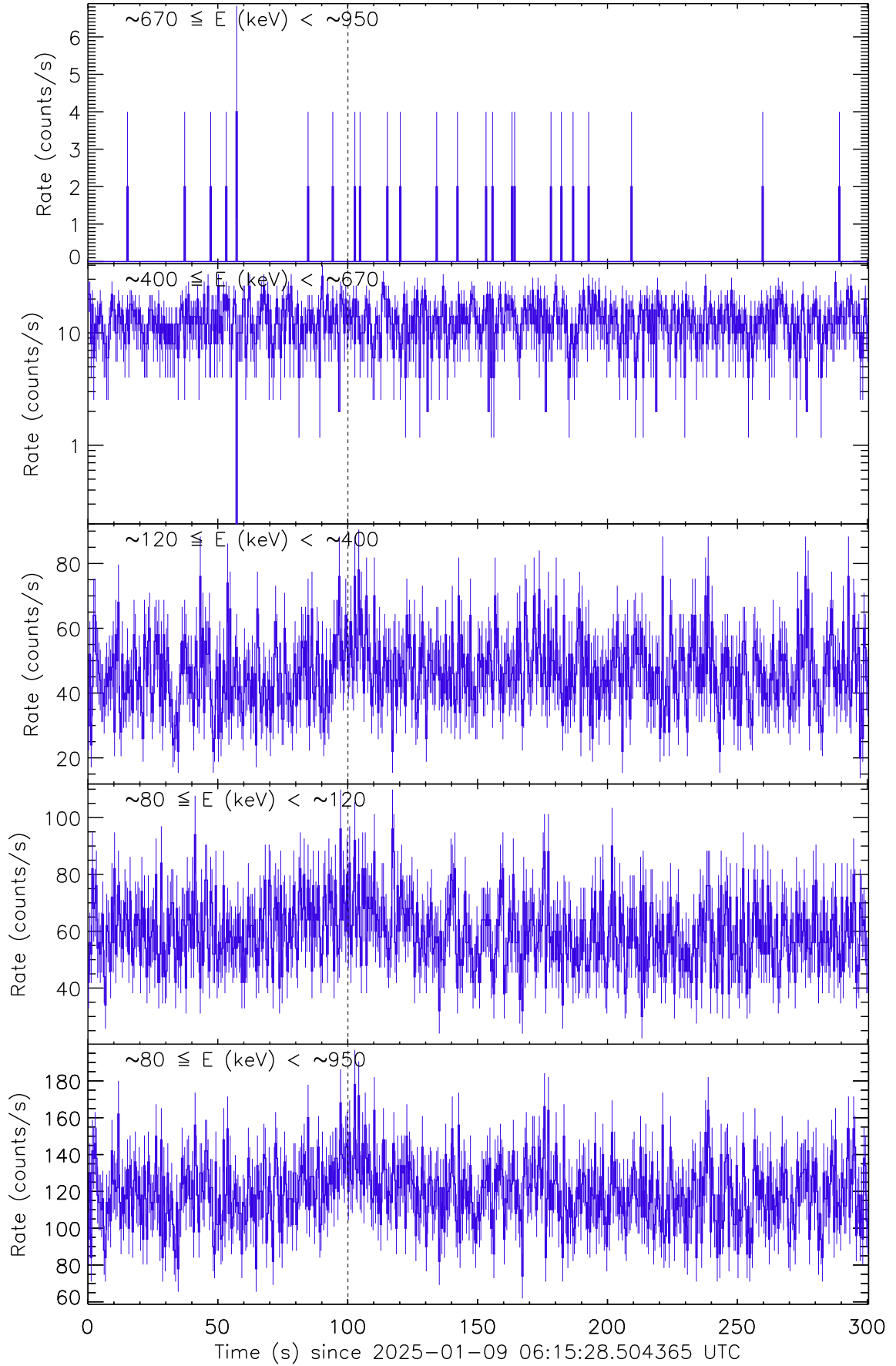
Figure 1: Raw count rate curve of GRB 250109A / EP250109a. The vertical dashed line marks the trigger time by Fermi/GBM.
