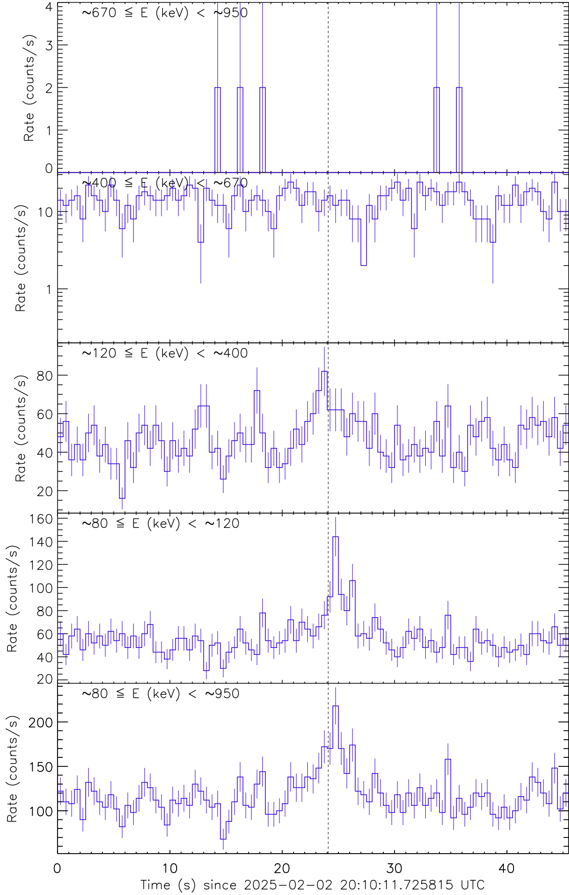
Figure 1: Raw count rate curve of GRB 250202C. The vertical dashed line marks the trigger time by Fermi/GBM.
